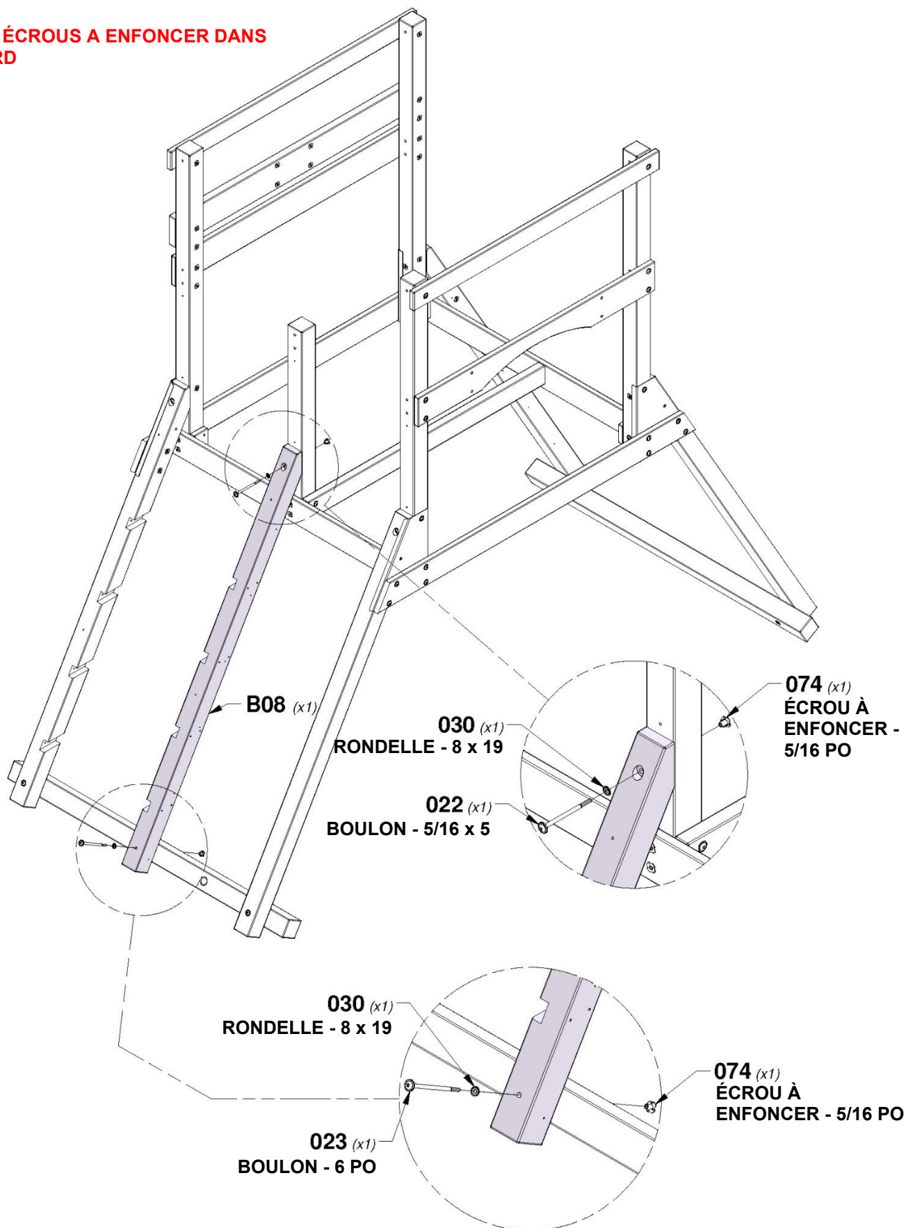
B08 | PIED - W4L16433
