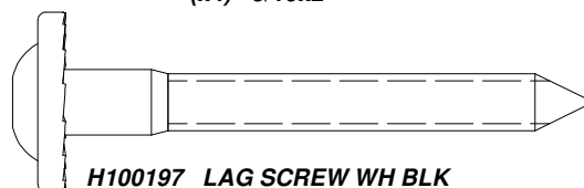
H100458 LAG SCREW WH BLK (x4) 5/16x2
