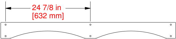
MT05 WALL RAIL - W4L21113 (x1) 5/8"x4 3/4"x51 1/4" (16x120x1303)
