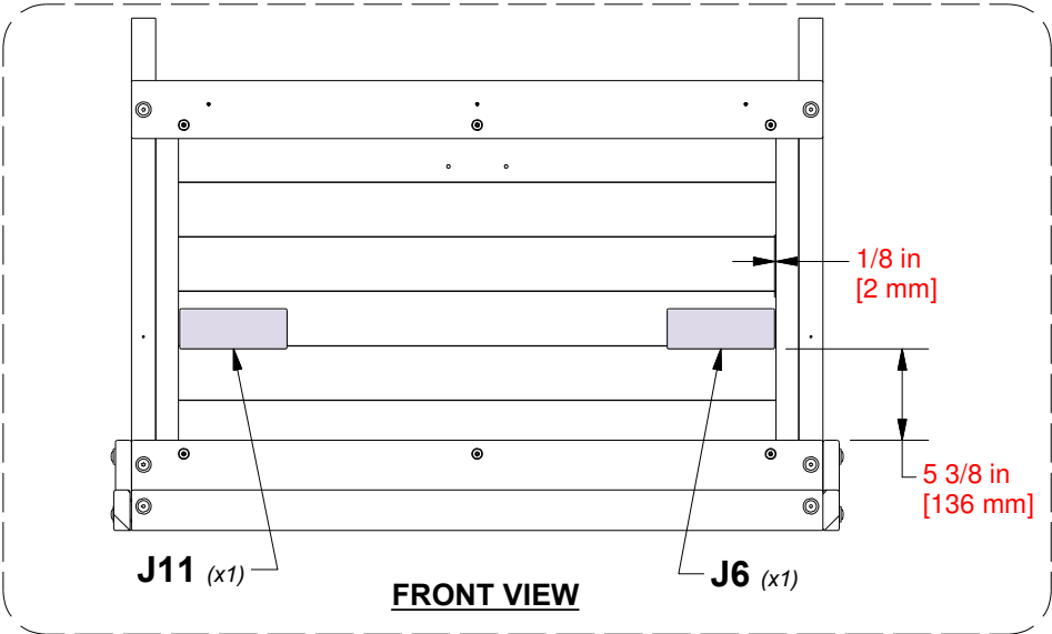
J6 SUPPORT BLOCK - W4L17817 (x1) 1"x2 3/8"x6 1/4" (24x60x160)
