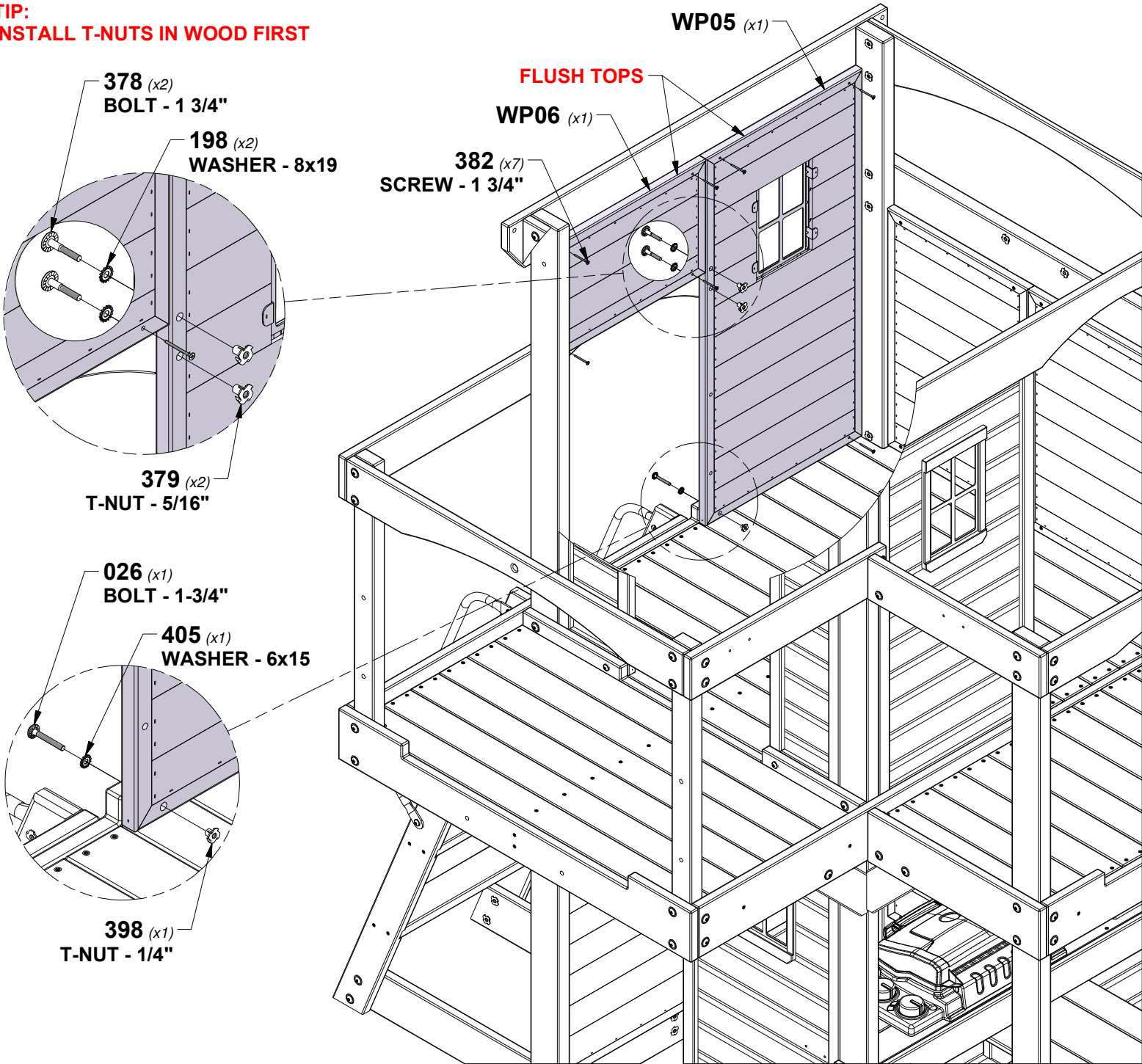
WP06 WALL PANEL - W2A03780 (x1) 1"x18 7/8"x11 3/4" (24x479x300)
