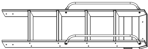
LADDER ASSEMBLY (x1)
