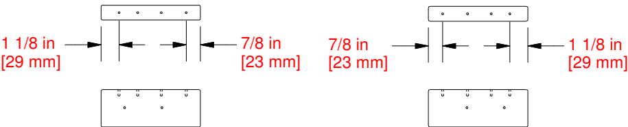
J6 SUPPORT BLOCK - W4L17817 (x1) 1"x2 3/8"x6 1/4" (24x60x160)
