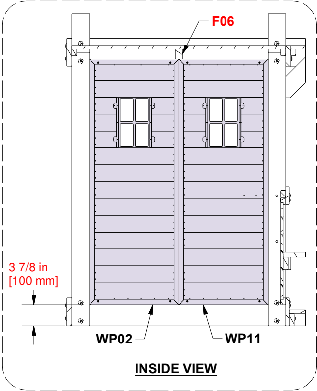
WP02 WALL PANEL - W2A03779 (x1) 1"x16 7/8"x46 1/2" (24x430x1181) WP11 WALL PANEL - W2A03788 (x1) 1"x16 7/8"x46 1/2" (24x430x1181)
