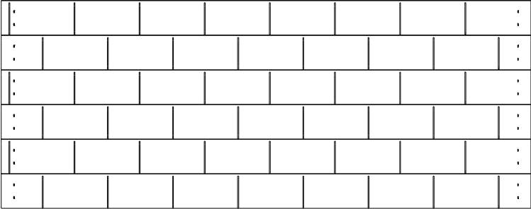
RP2 TOP ROOF PANEL - W2A04025 (x2) 1 3/8"x19 1/8"x48 5/8" (35x486x1236)
