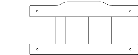
WP10 BENCH BACK ASSEMBLY - W2A037777 (x1) 1 1/8"x11 7/8"x24 1/4" (27x303x615)
