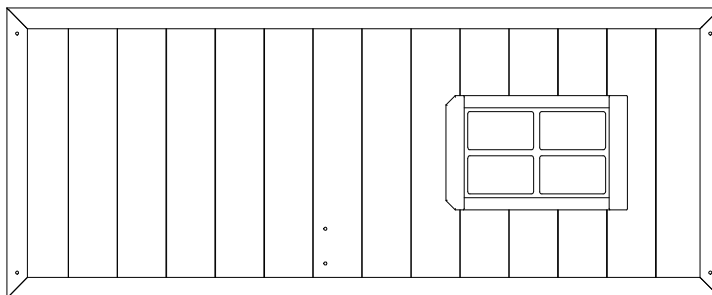
WP12 WALL PANEL - W2A03789 (x1) 1"x16 7/8"x46 1/2" (24x479x1181)
