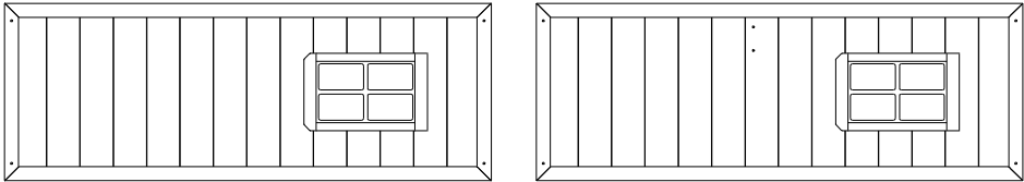
WP02 WALL PANEL - W2A03779 (x1) 1"x16 7/8"x46 1/2" (24x430x1181) WP11 WALL PANEL - W2A03788 (x1) 1"x16 7/8"x46 1/2" (24x430x1181)
