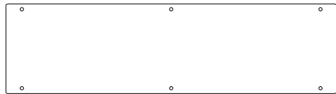
K03 BOTTOM - W4L19825 (x1) 5/8"x5 1/4"x19 1/2" (16x134x495)
