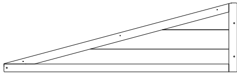
WP08 WALL PANEL - W2A04147 (x1) 1"x11 3/8"x38 3/8" (24x290x975)
