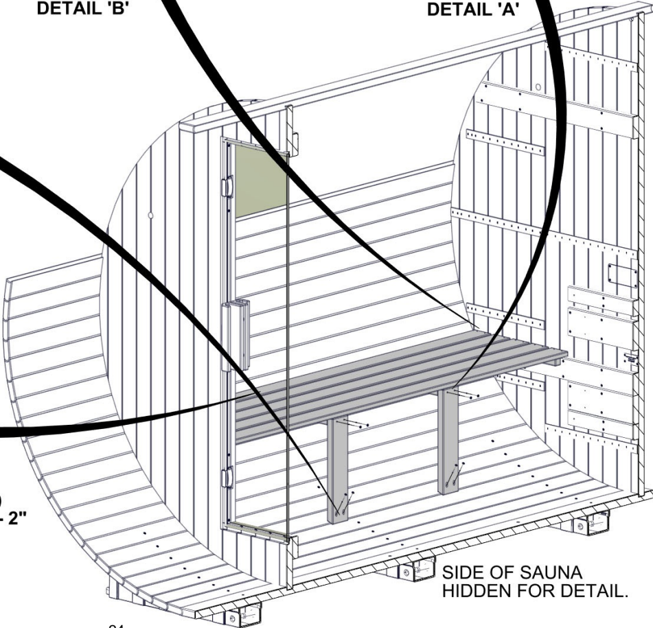
1443 (x4) SCREW - 1 1/2" OG04 (x2) BENCH BRACE
