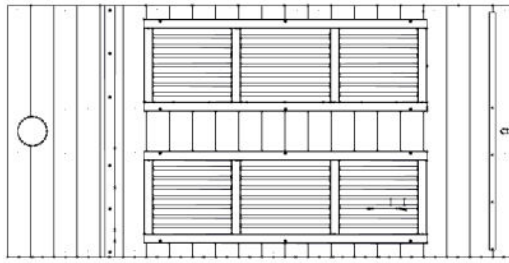
P02 BACK WALL PANEL - W2A04860 (x1) 2 11/16"x36"x72 13/16" (69x914x1850)
