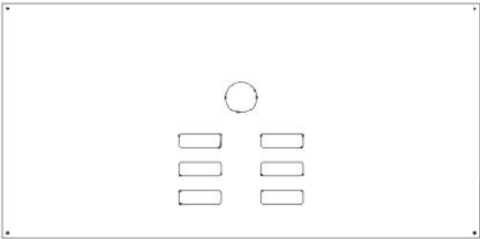
R01 ROOF COVER - W2A04864 (x1) 3/16"x17 11/16"x35 13/16" (5x450x910)
