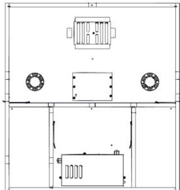
P08 ROOF PANEL - W2A04861 (x1) 158"x14 1/16"x35 13/16" (4014x357x910)
