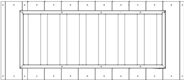
P05 SEAT SUPPORT PANEL - W2A04862 (x1) 1 7/8"x15 3/8"x35 13/16" (48x390x910)
