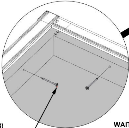
382 (x8) SCREW - 1 3/4"
