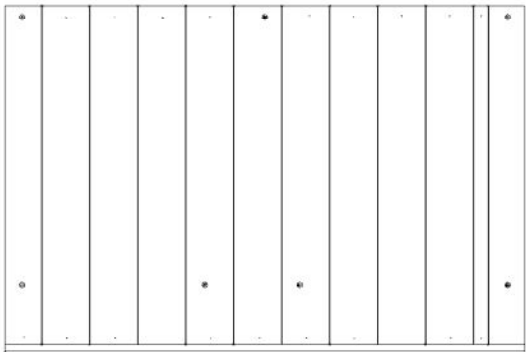
P06 SEAT PANEL - W2A04865 (x1) 1 3/4"x23 13/16"x44 3/4" (44x605x1136)
