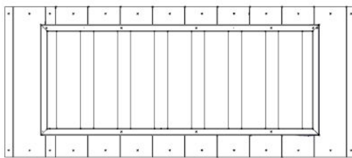
P05 SEAT SUPPORT PANEL - W2A04862 (x1) 1 7/8"x15 3/8"x35 13/16" (48x390x910)
