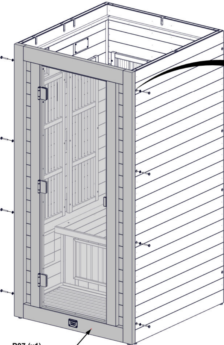
P07 (x1) FRONT PANEL
