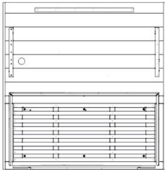
P01 FLOOR PANEL - W2A04859 (x1) 4 5/8"x40 1/16"x36" (118x1018x986)
