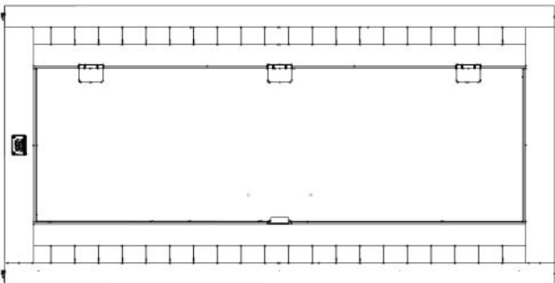
P07 FRONT PANEL - W2A04858 (x1) 1 7/16"x38 13/16"x76 9/16" (36x986x1944)
