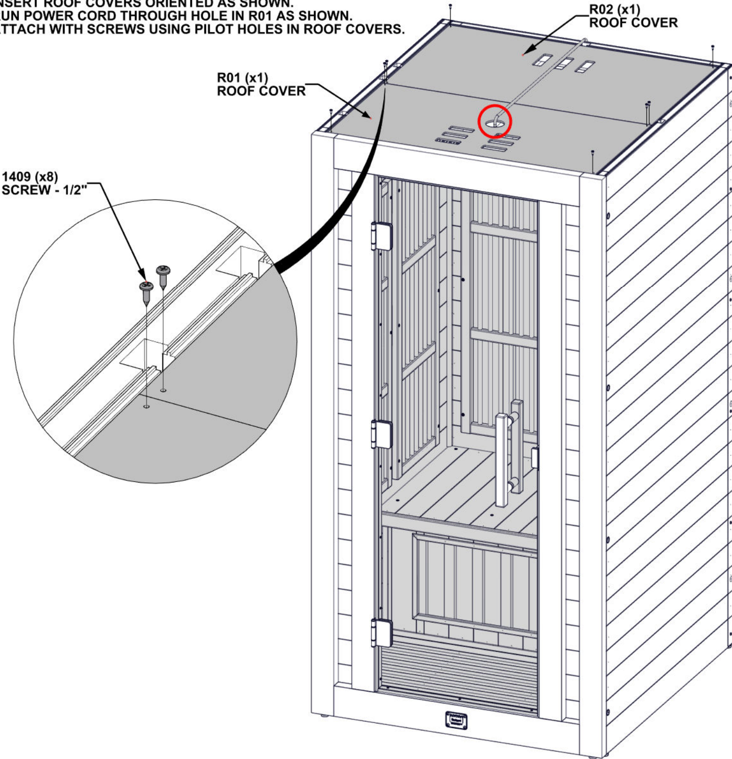
R01 ROOF COVER - W2A04864 (x1) 3/16"x17 11/16"x35 13/16" (5x450x910)
