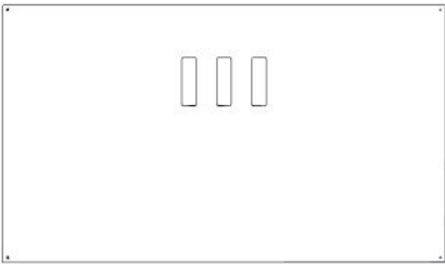
R02 ROOF COVER - W2A04863 (x1) 3/16"x20 7/8"x35 13/16" (5x530x910)
