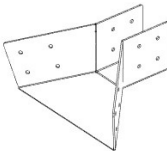
A4M01895 PANEL SUPPORT BRACKET (x2)
