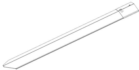
A4M02867 RIDGE CAP SPLICE ASSEMBLY (x4)
