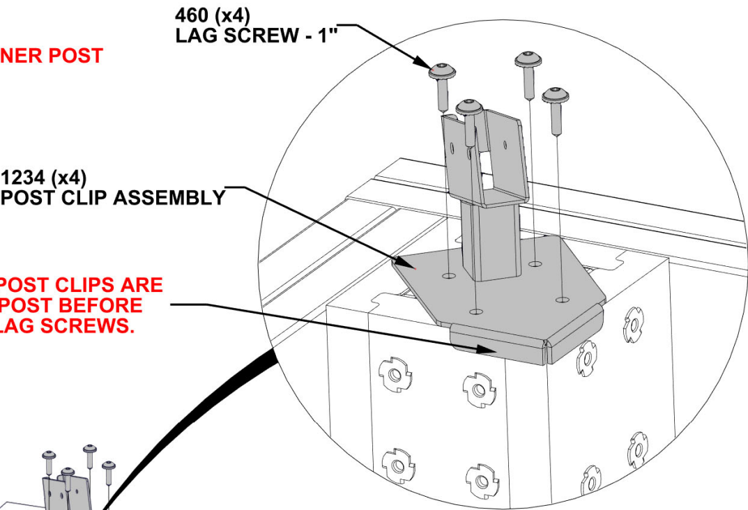
A4M01234 POST CLIP ASSEMBLY (x4)
