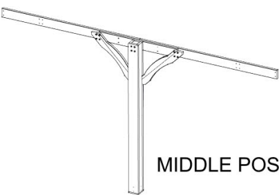
12FT BEAM ASSEMBLY
