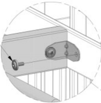
222 (x2) BOULON - 3/4 "
