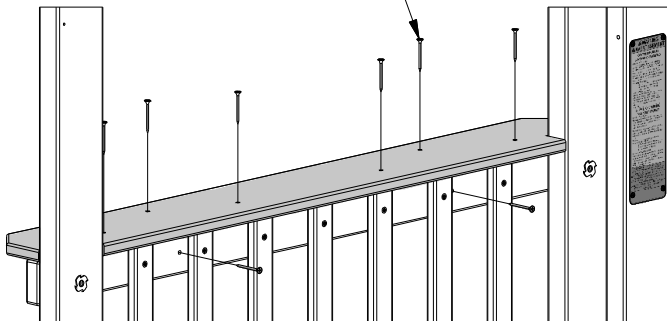
BACK VIEW
