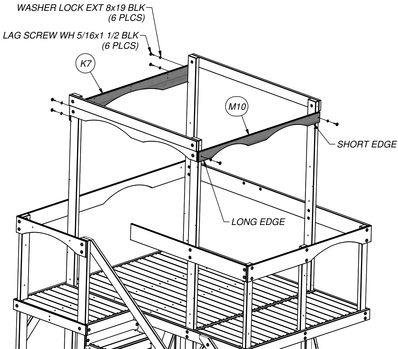
WASHER LOCK EXT (6) 8x19 BLK
