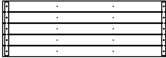
(1) FP1 - PANNEAU DE PLANCHER - W2A01679 1 5/8"x17 1/8"x50 1/4" (40x434x1276)
