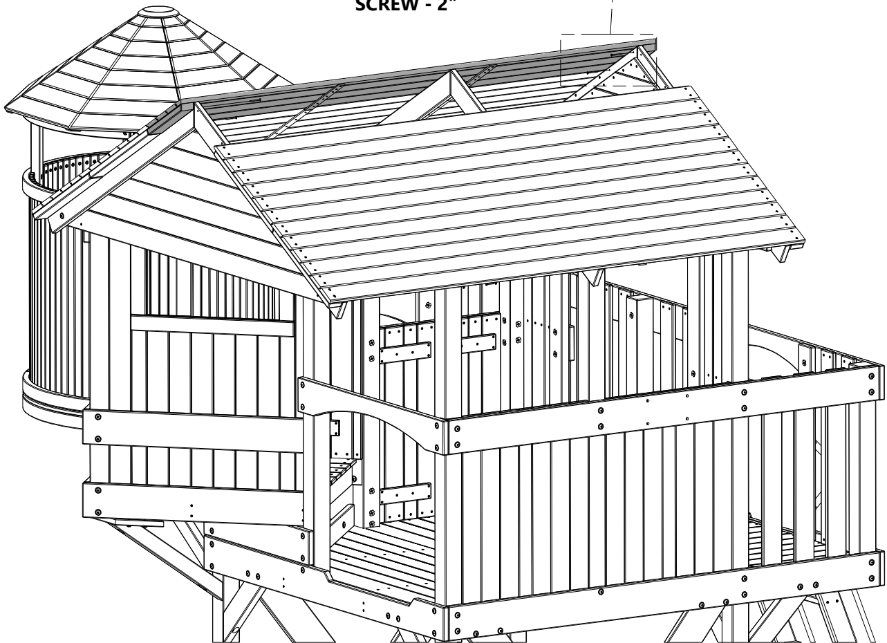
391 (x4) SCREW - 2"
