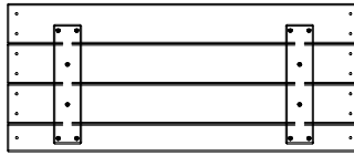
WP2 | RIGHT WALL PANEL - W2A02904 (x2) | 1 1/4"x12 1/2"x29 7/8" (32x318x759)
