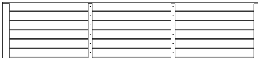
RP02 | ROOF PANEL - W2A020184 (x2) | 1 9/16"x19 1/4"x85 3/16" (40x488x2165)
