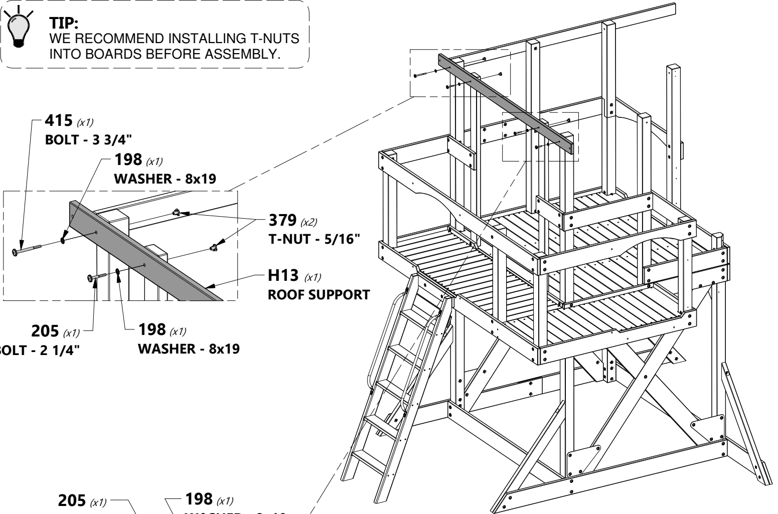
H100205 | BOLT WH BLK (x2) | 5/16x2-1/4
