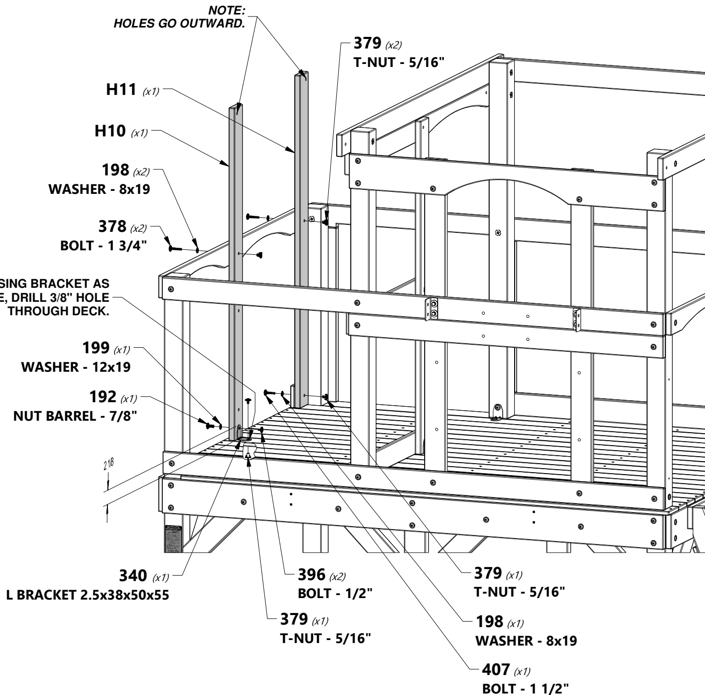
H100192 | NUT BARREL WH (1) BLK 5/16x7/8
