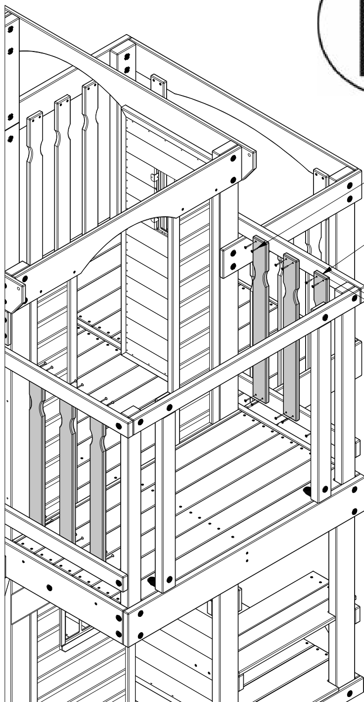
088 (x24) SCREW - 1 1/8"
