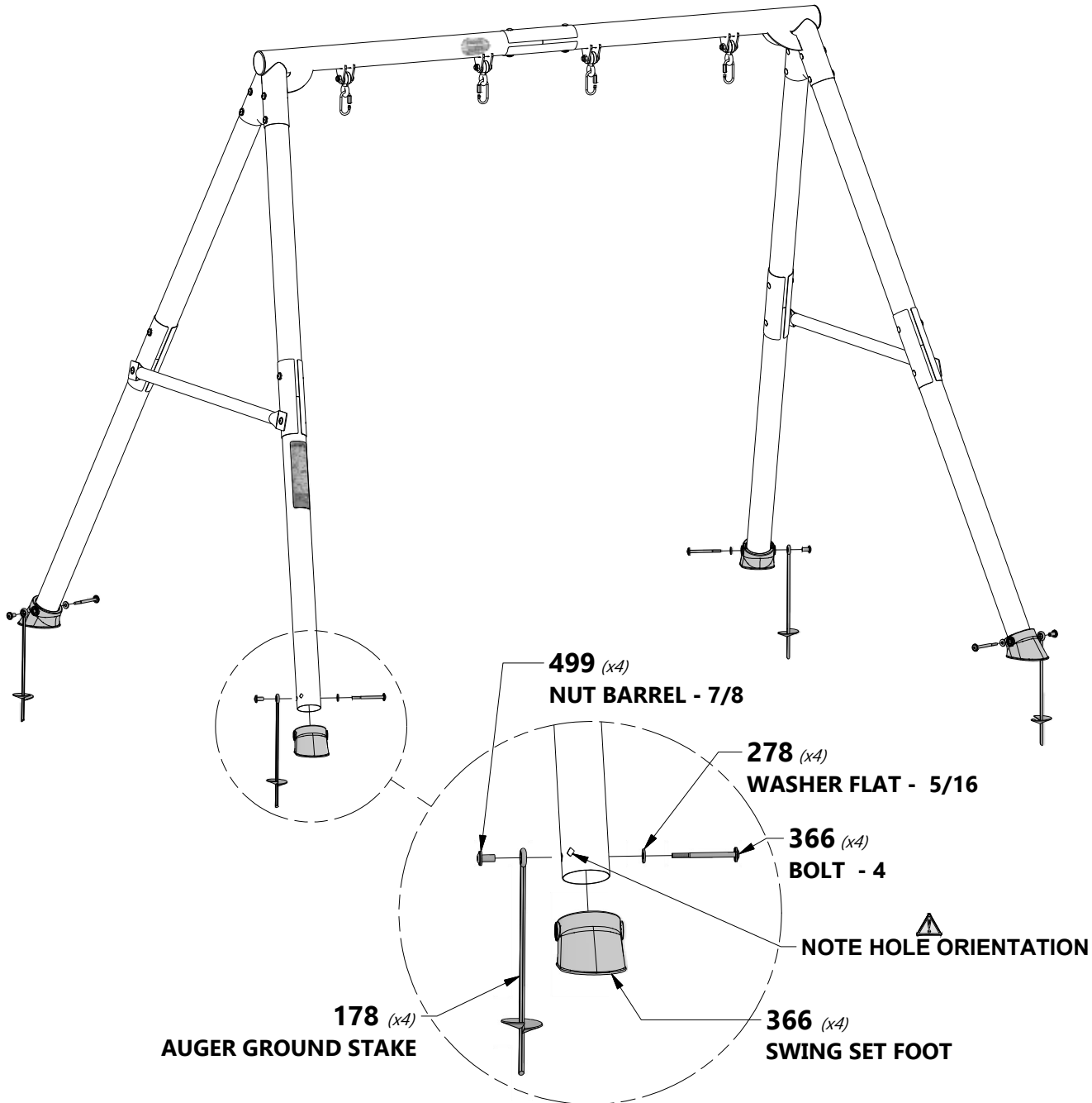
H100499 (x4) | NUT BARREL WH WZ 5/16x7/8
