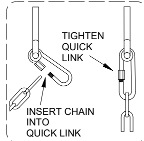
H100242 (x4) | QUICK LINK (LONG) WZ
