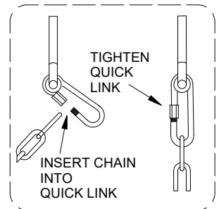
H100242 (x4) | QUICK LINK (LONG) WZ
