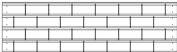
RP1 | PANEL INFERIOR DEL TECHO - W2A03166 (x2) | 1 3/8 "x13" x44 7/8 "(35x329x1140)
