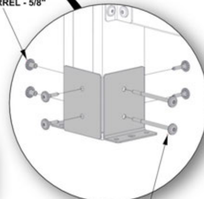
480 (x8) BOLT - 4 3/4"
