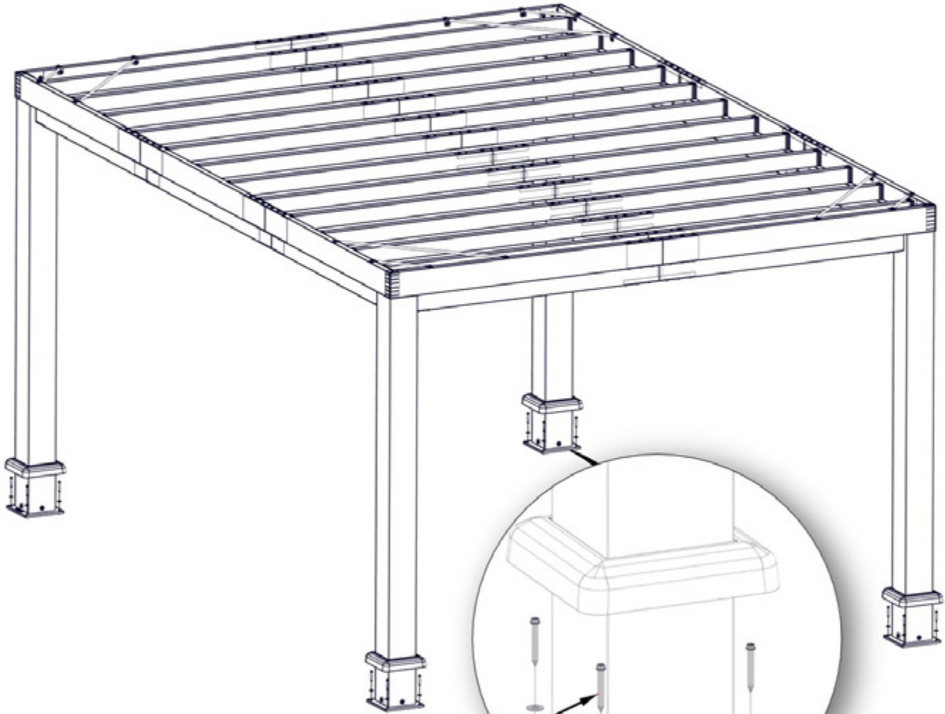
120 (x16) SCREW - 2"
