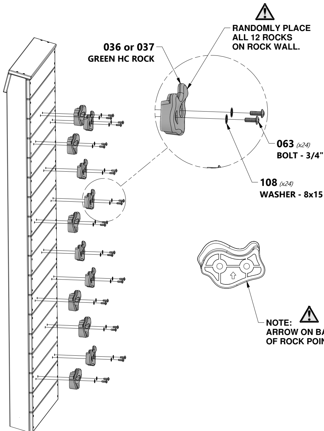
A6P00037 | GREEN HC ROCK #2 (x6)
