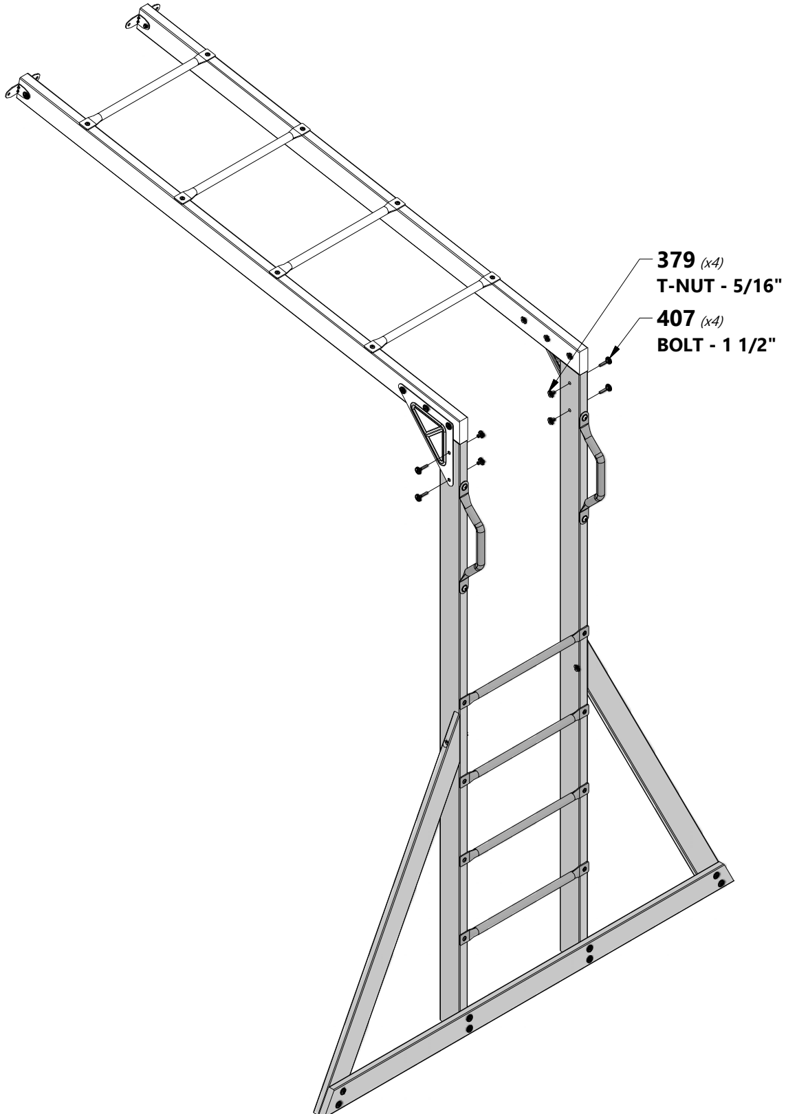
H100407 | BOLT WH BLK (x4) | 5/16x1 1/2
