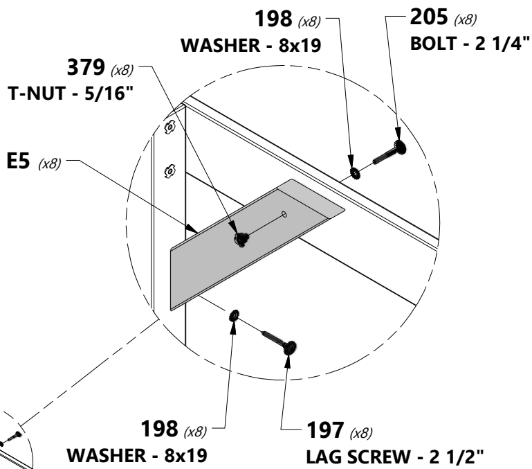
H100379 | T-NUT BLK (x8) 5/16
