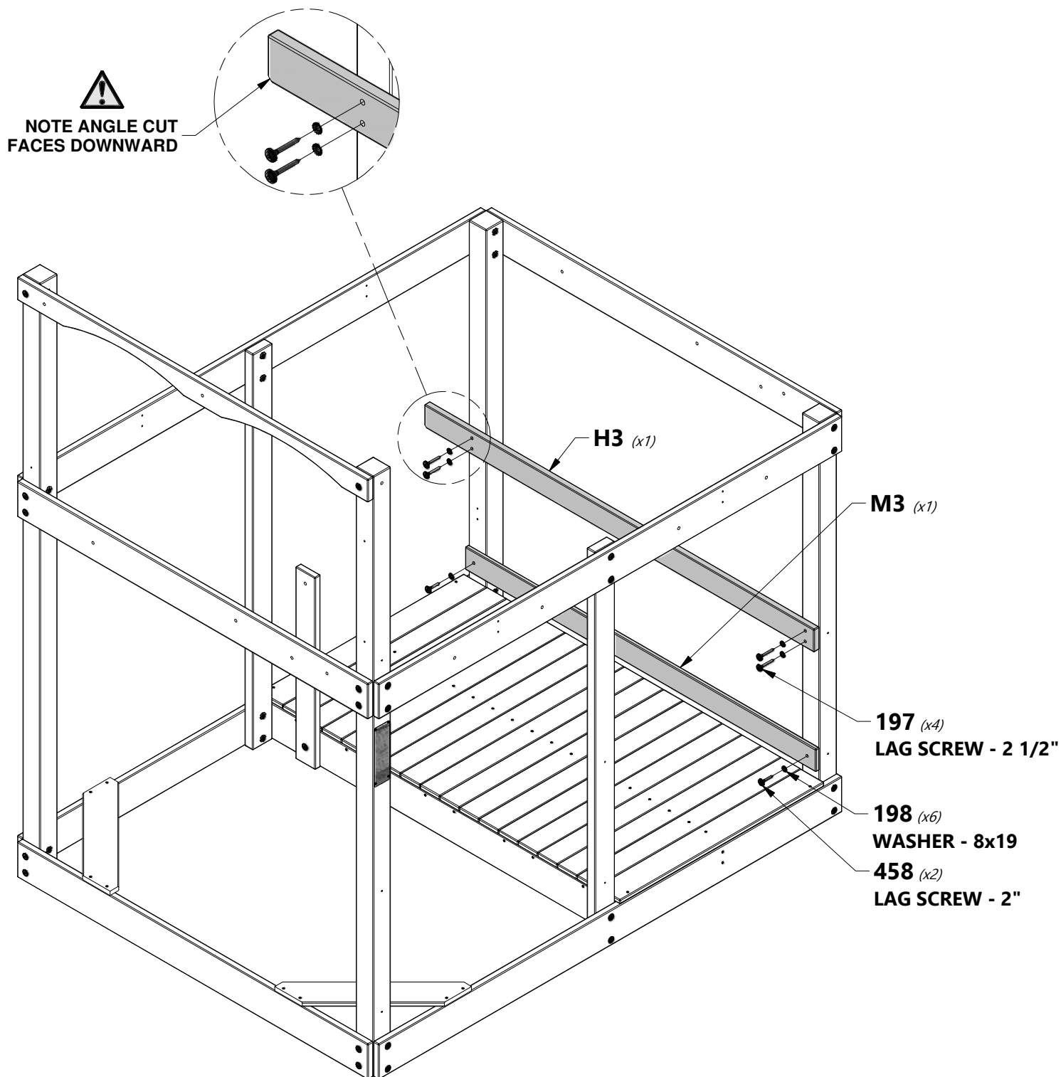
H100197 | LAG SCREW WH BLK (x4) | 5/16x2 1/2
