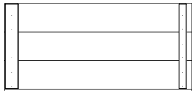
RP2 | LEFT PORCH ROOF PANEL - W2A03143 (x1) | 1 5/8"x15 5/8"x32 7/8" (42x396x834)
