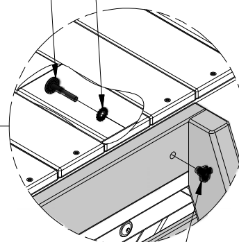
379 (x2) T-NUT - 5/16"
