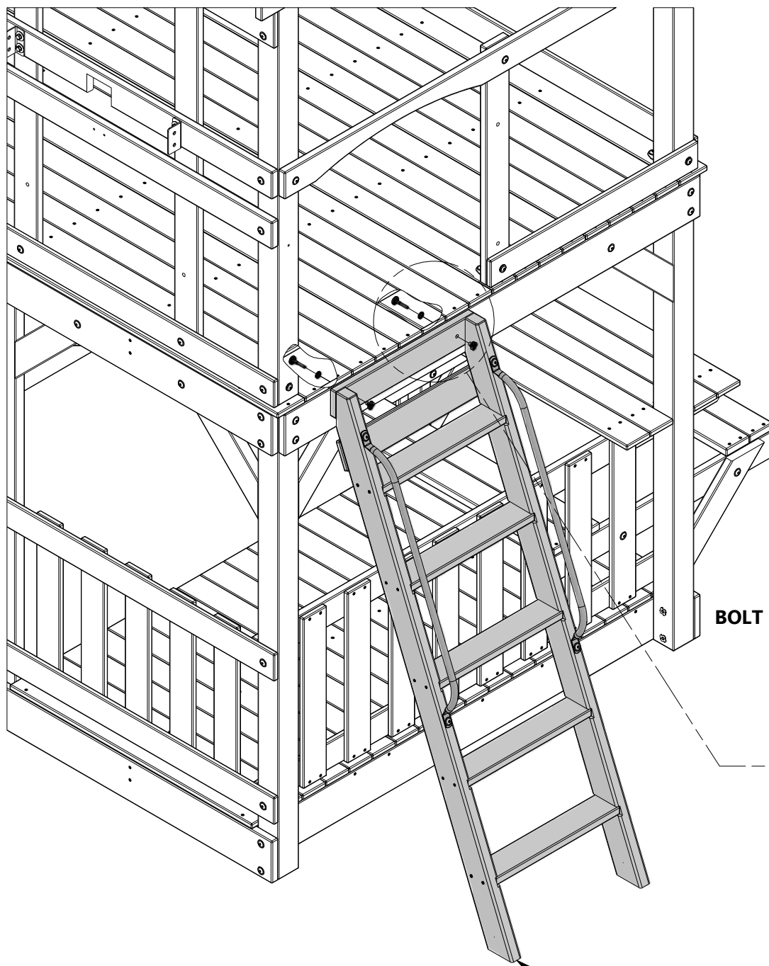
LADDER ASSEMBLY
