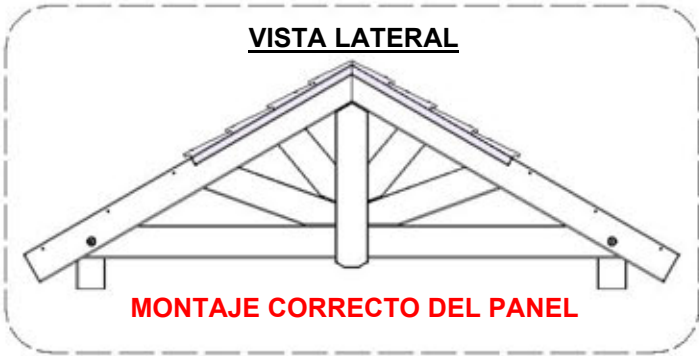
RP1 | PANEL SUPERIOR DEL TECHO - W2A03276 (x2) 1 5/8"x20 5/8"x59" (42x511x1676)
