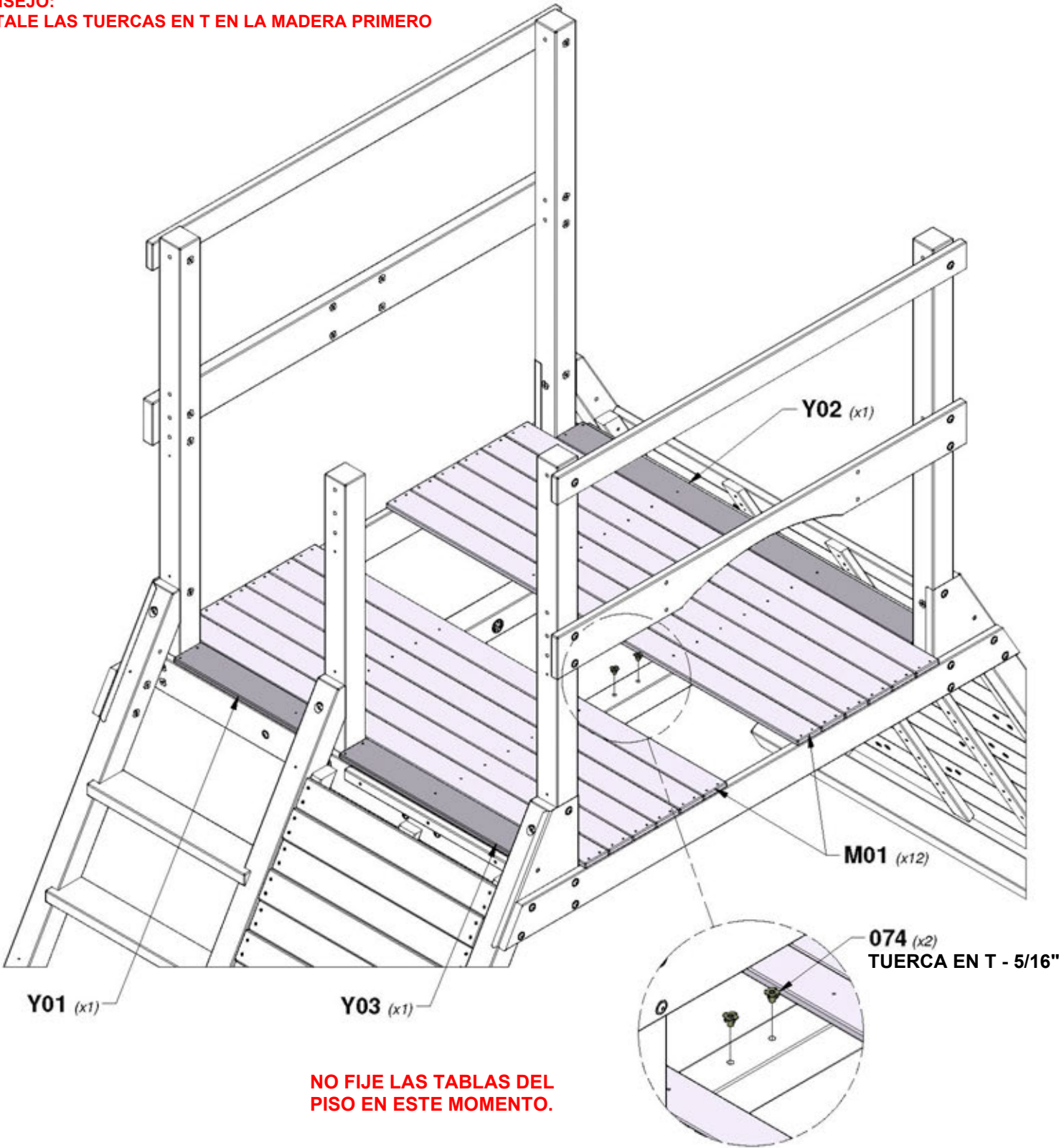
Y02 | TABLA DE PISO - W4L15745 (x1) 5/8"x4"x51 1/2" (16x102x1307)
