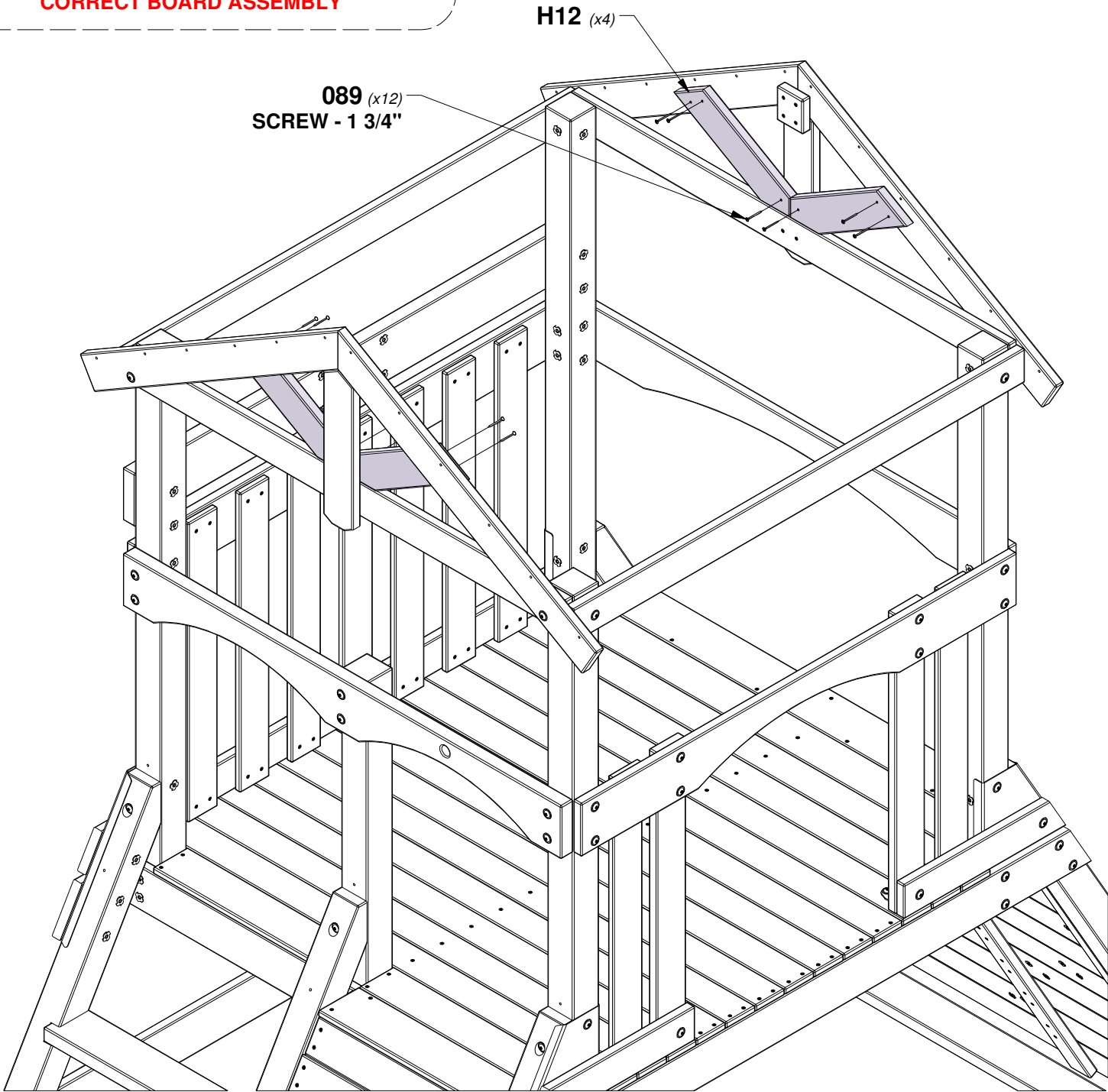
CORRECT BOARD ASSEMBLY
