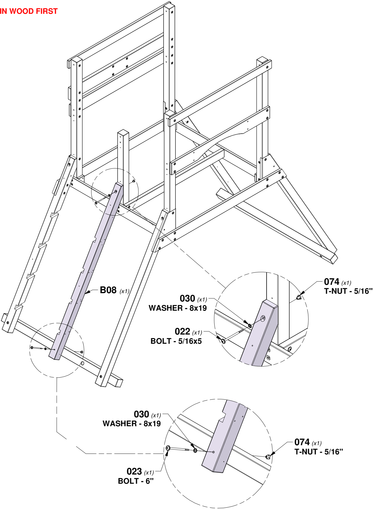
B08 | LEG - W4L16433 (x1) | 3"x3"x69 1/4" (76x76x1760)
