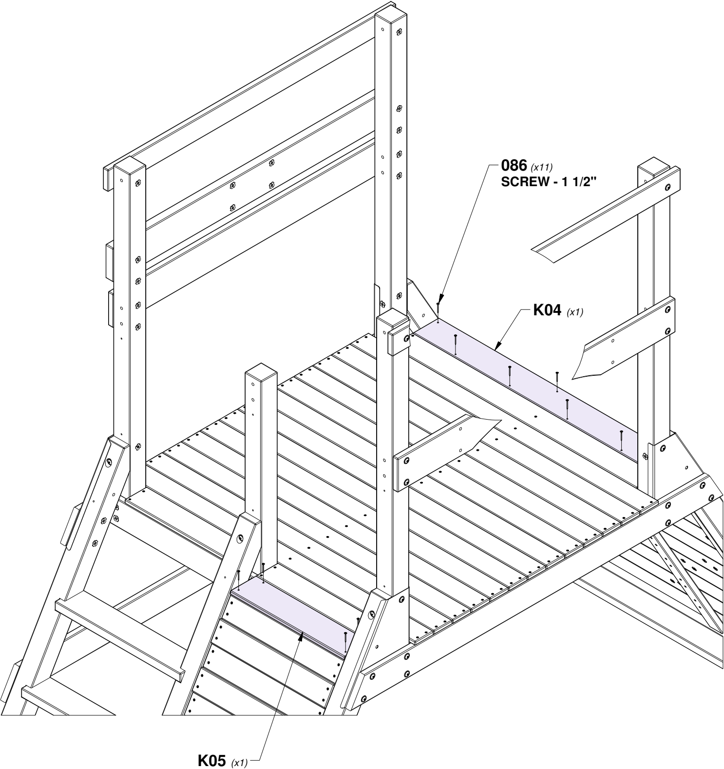
K05 FLOOR BOARD - W4L16449 (x1) 5/8"x4 3/4"x20 7/8" (16x120x529)
