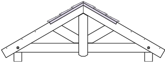
CORRECT PANEL ASSEMBLY
