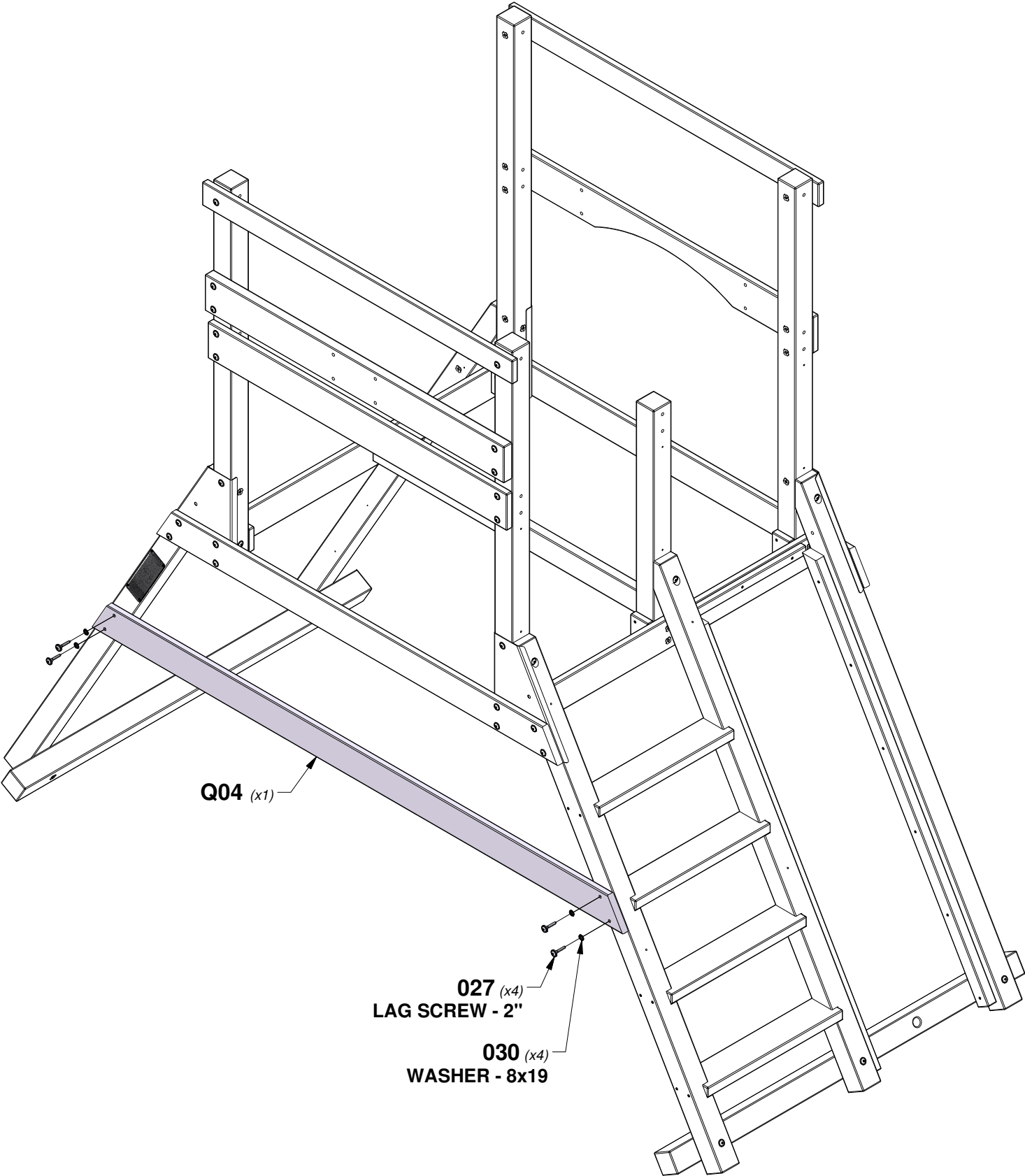
Q04 | SAFETY RAIL - W4L16475 (x1) 1"x4 3/8"x89 1/2" (24x112x2274)
