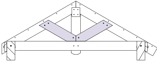
CORRECT BOARD ASSEMBLY
