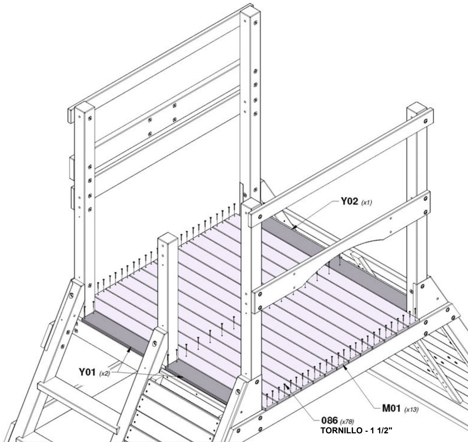
Y02 | TABLA DEL PISO - W4L16439 (x1) 5/8"x4"x44 5/8" (16x102x1135)
