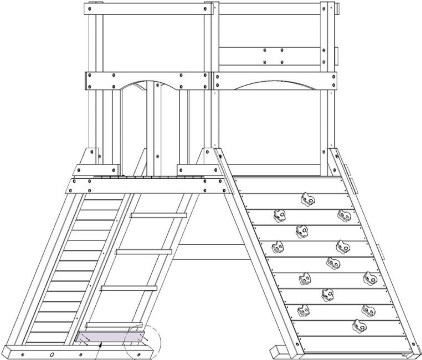
M05 (x1)
