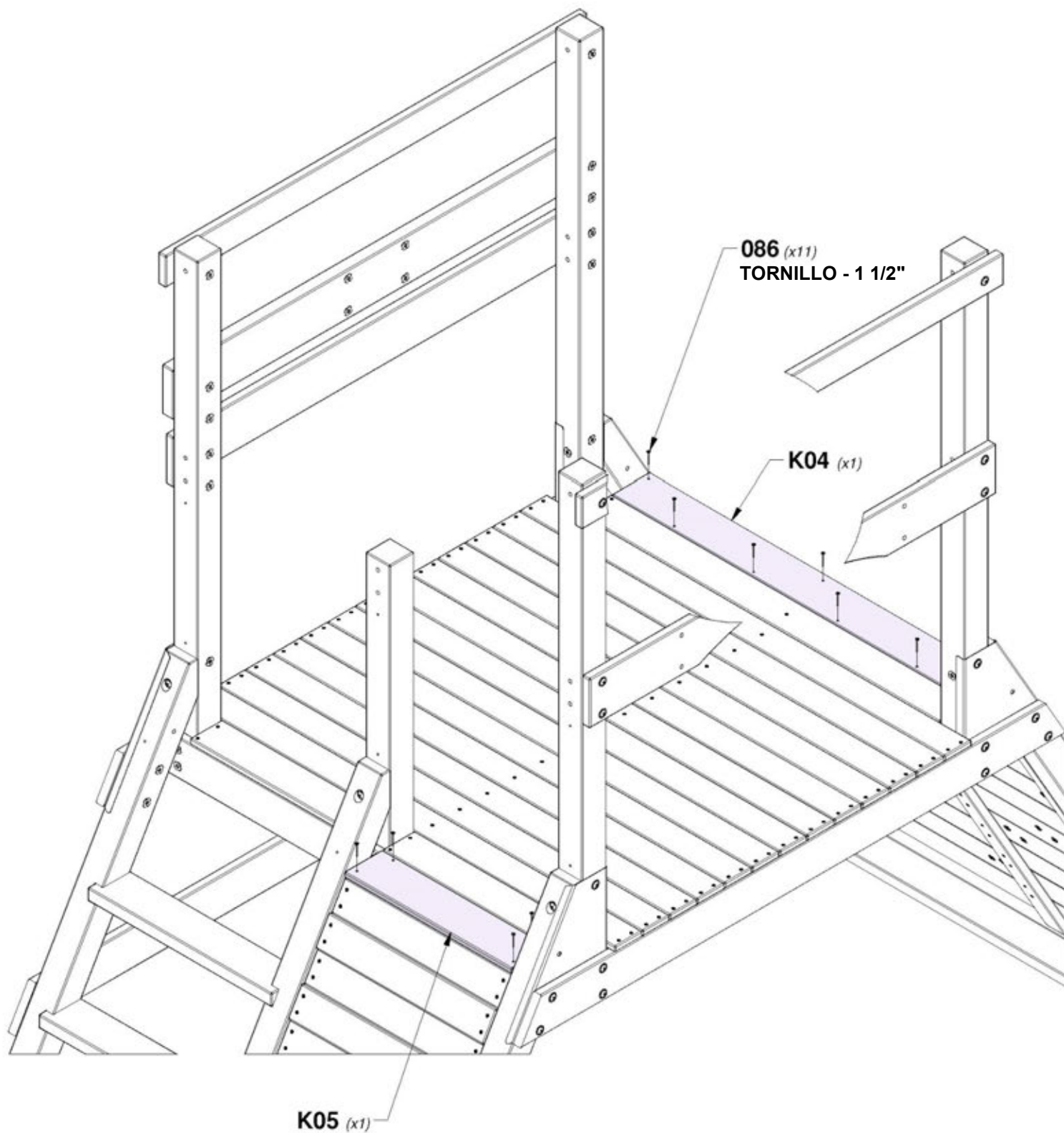
K05 TABLA DEL PISO - W4L16449 (x1) 5/8"x4 3/4"x20 7/8" (16x120x529)
