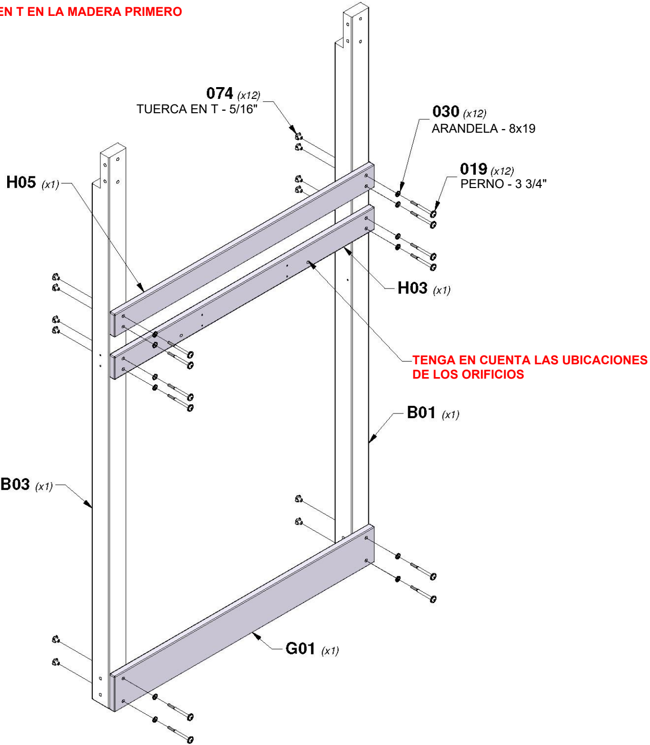
B03 MONTANTE - W4L16126 (x1) 3"x3"x82 1/4" (76x76x2089)
