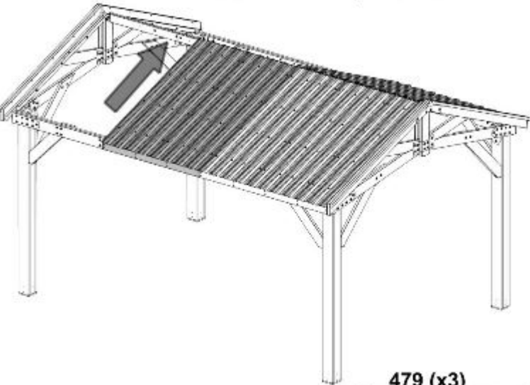
INSTALL ROOF PANEL A, SECTION 2
