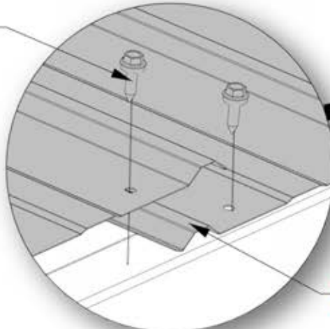
117 (x80) SCREW - 3/4"
