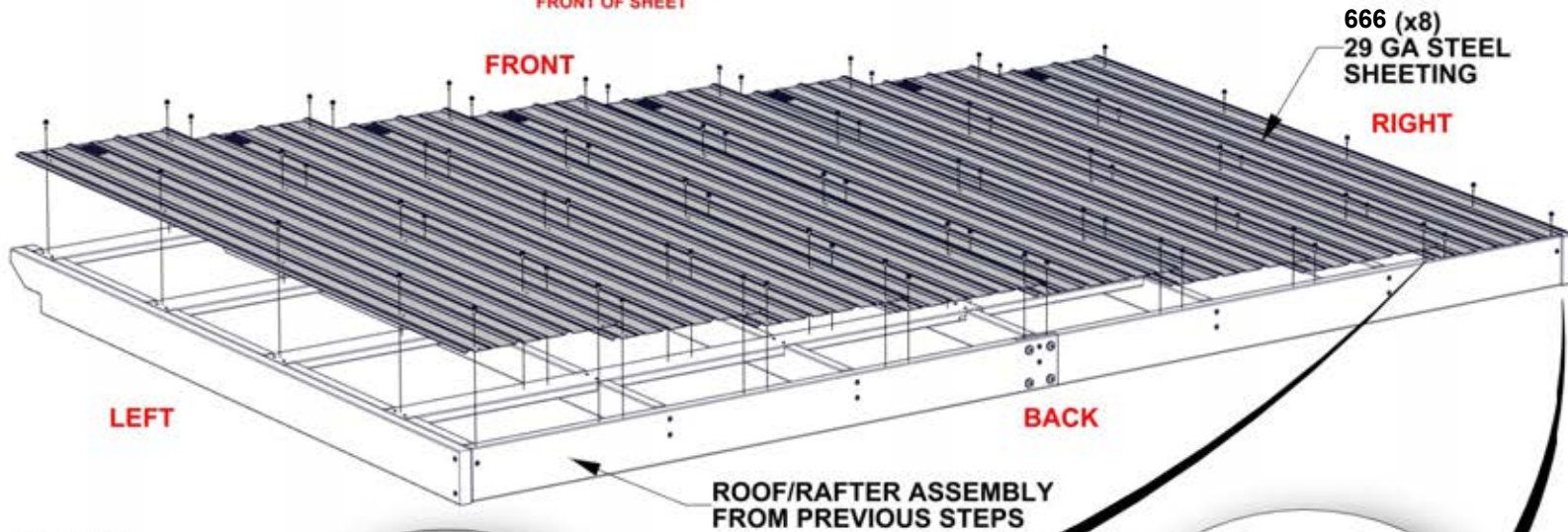
117 (x80) SCREW - 3/4"
