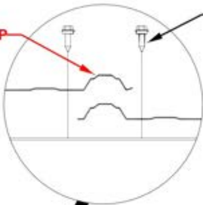
833 (x32) SCREW-3/4"
