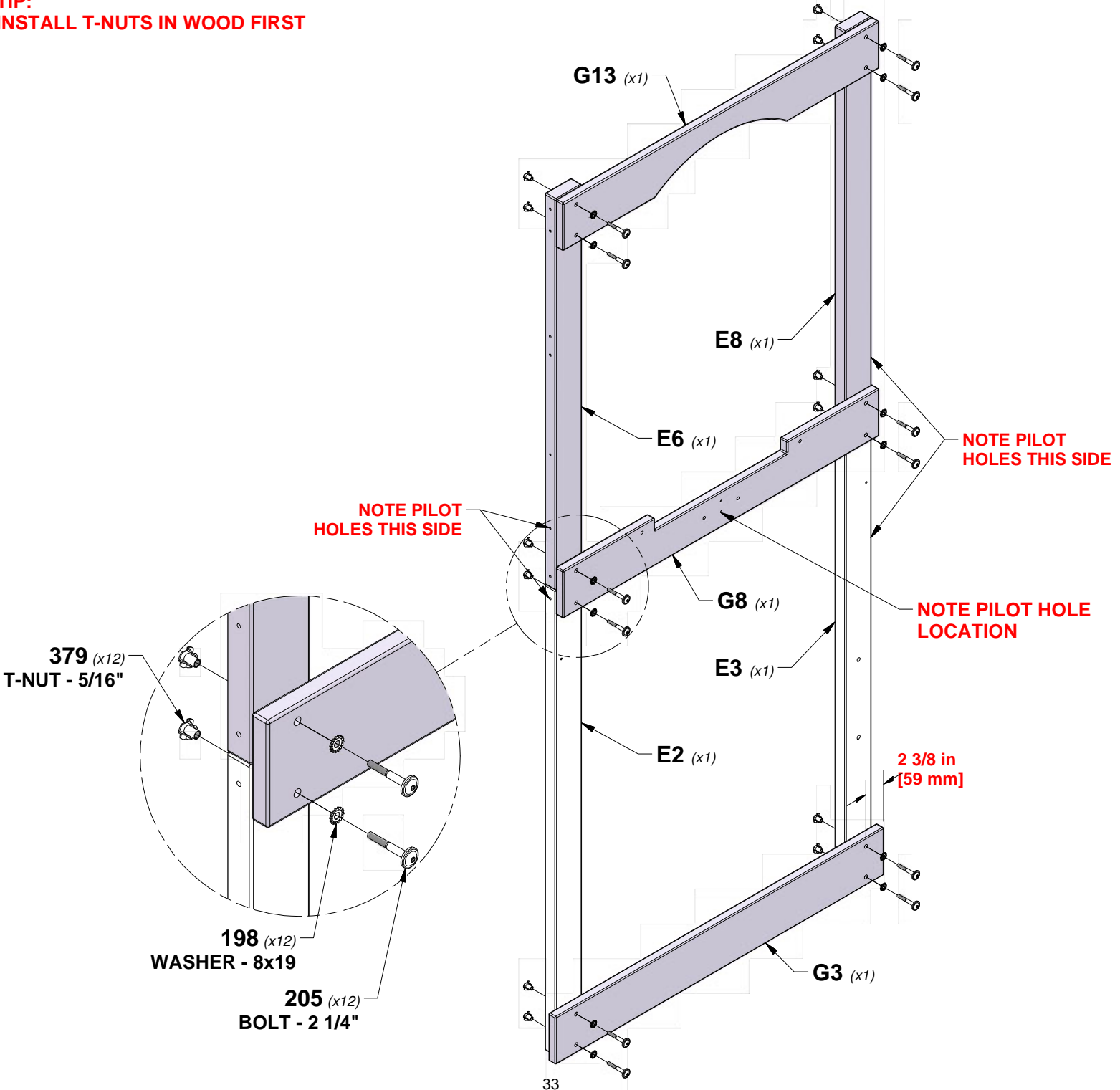
G8 LEFT CENTER WALL RAIL - W4L19000 (x1) 1"x5 1/4"x40 5/8" (24x134x1032)
