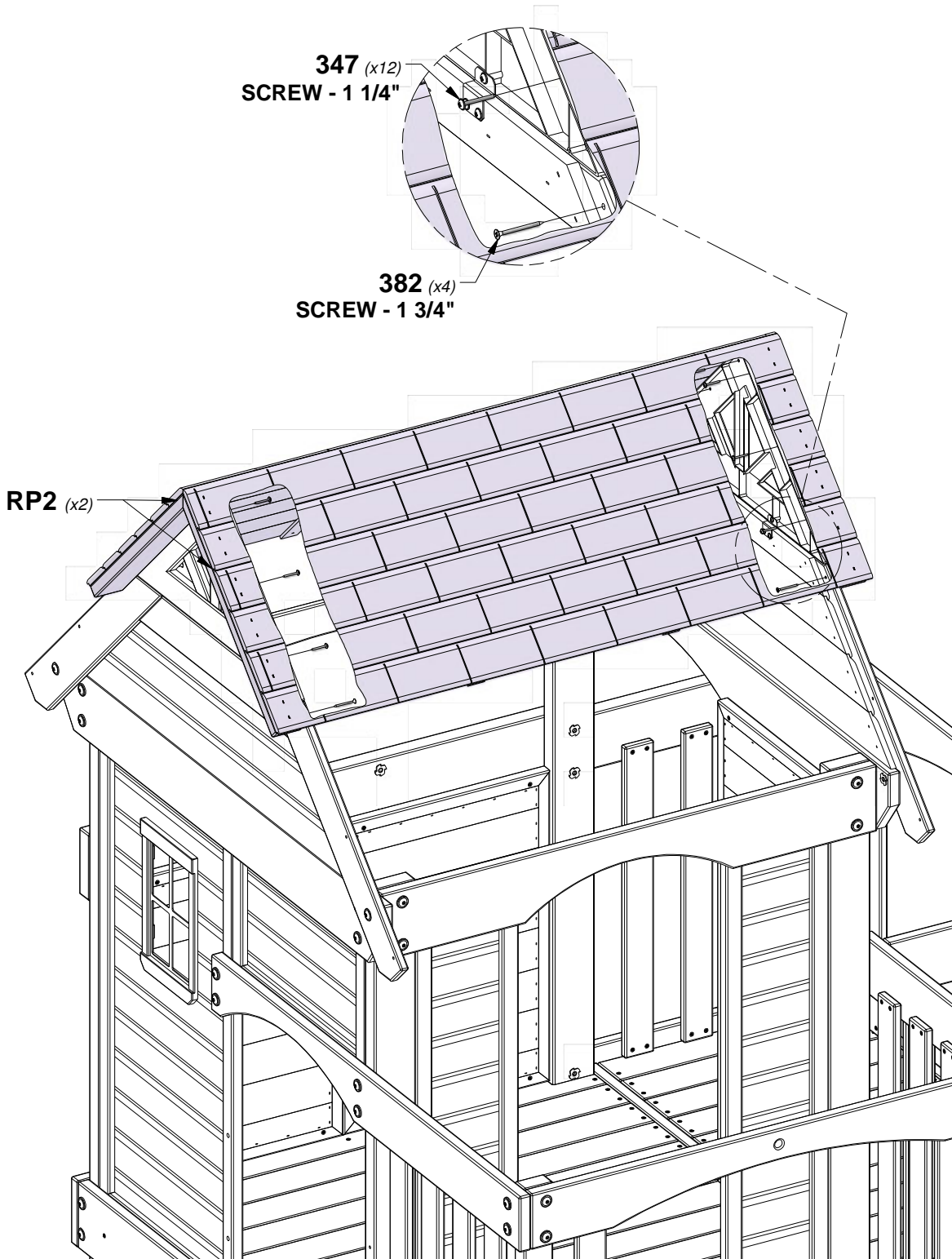
RP2 TOP ROOF PANEL - W2A04025 (x2) 1 3/8"x19 1/8"x48 5/8" (35x486x1236)
