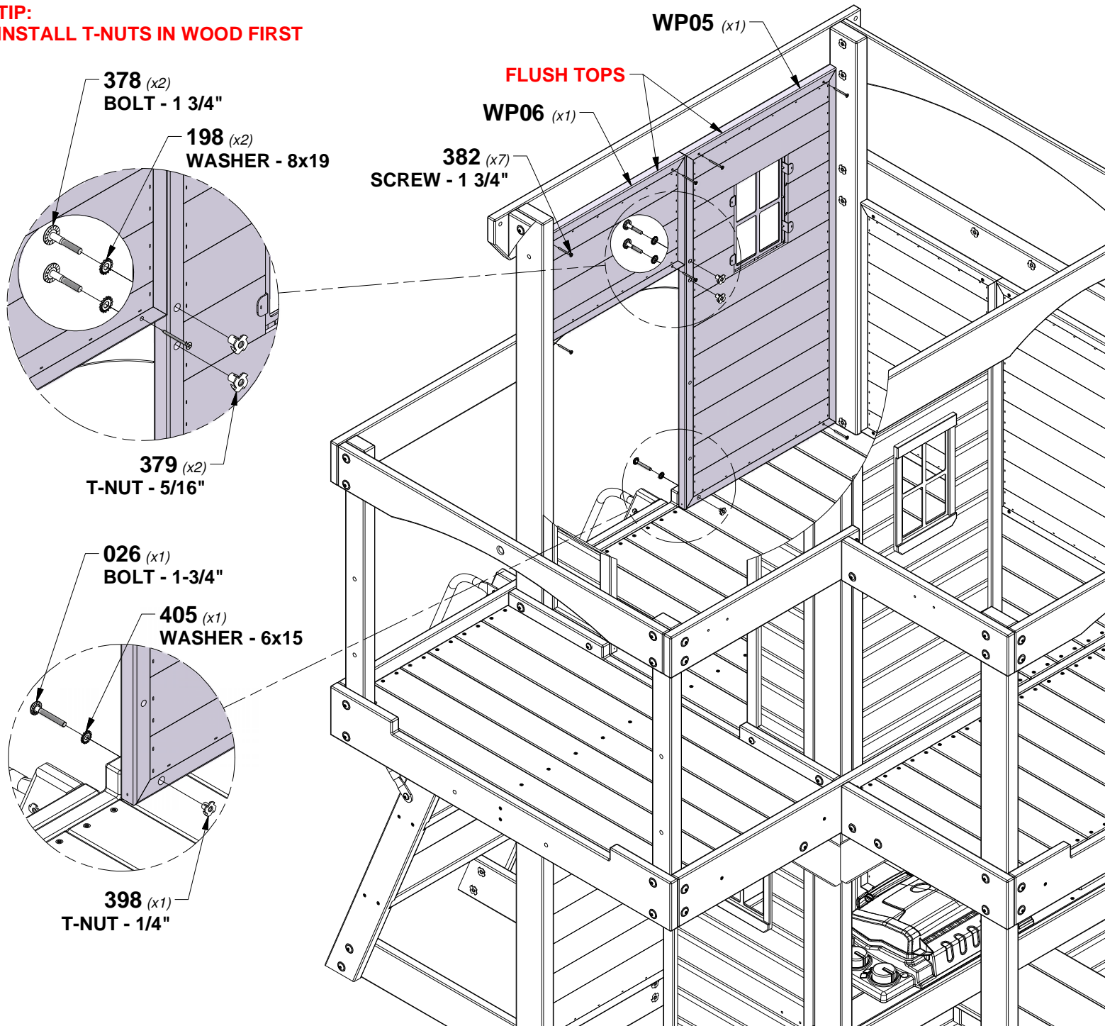
WP06 WALL PANEL - W2A04104
