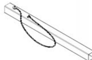
T03 UPRIGHT TUBE WITH MATCH HOLDER - A4M02404 (x1) 1 9/16"x1 9/16"x22 11/16" (40x40x576)
