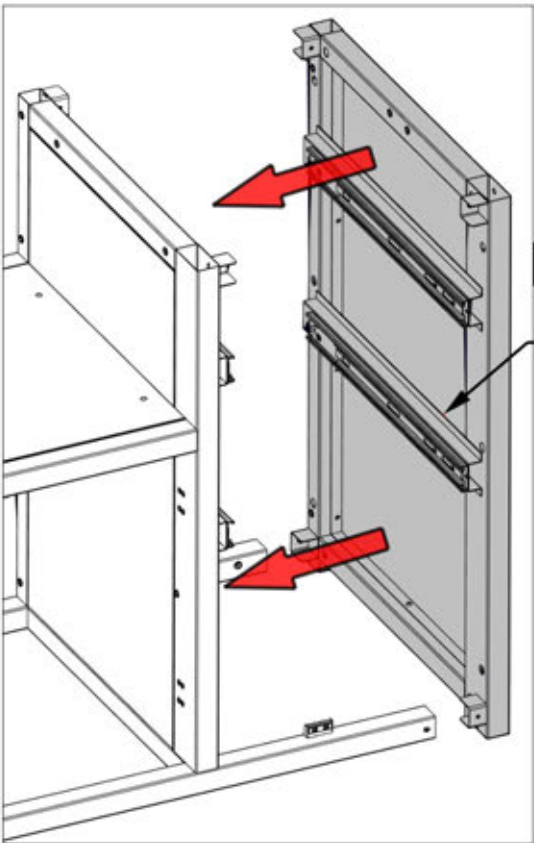
C06 (x1) CABINET PANEL
