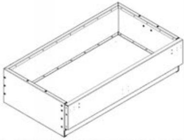
C01 COAL PAN ASSEMBLY - A4M02135 (x1) 1 15/16"x25 1/4"x44 13/16" (292x642x1139)
