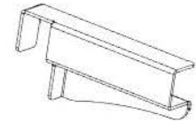
SHELF SUPPORT LEFT - A4M02547 (x3)
