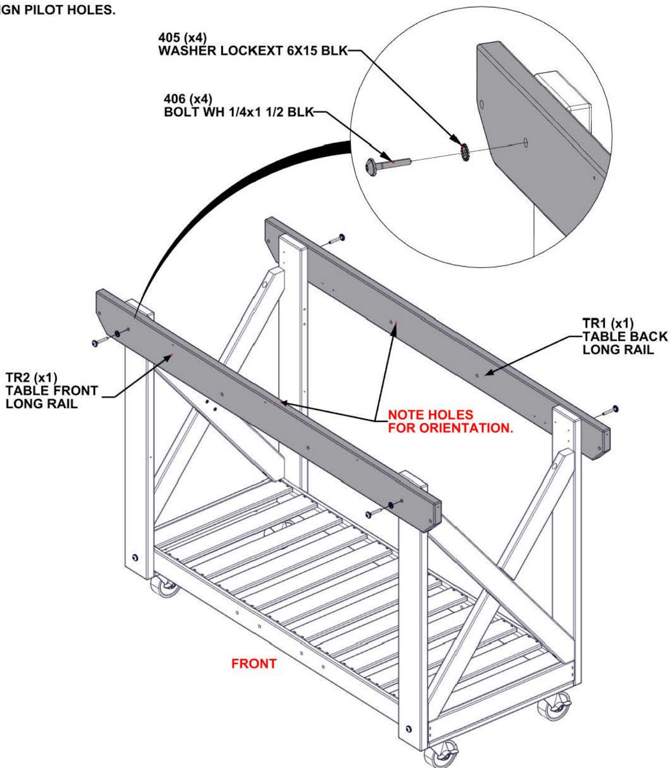
TR2 - TABLE FRONT LONG RAIL- W4L18895 (x1) 15/16"x4"x50 11/16" (24x102x1287)
