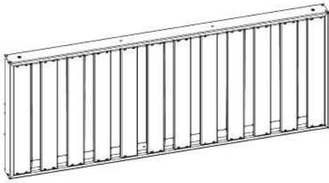
BP1 - BOTTOM PANEL - W2A04015 (x1) 2 3/8"x18"x44 5/16" (60x458x1125)
