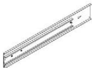
A10 ASSEMBLAGE DE SUPPORT DE GLISSIÈRE - A4M03083 (x2) 15/16"x3 3/8"x22 5/8" (23x85x575)
