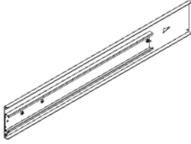
A10 MONTAGE DU SUPPORT DE GLISSIÈRE - A4M03083 (x6) 15/16"x3 3/8"x22 5/8" (23x85x575)
