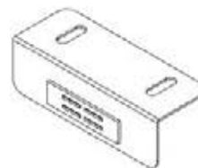
A2 SUPPORT MAGNÉTIQUE- A4M03026 (x1) 1"x1 1/4"x3 1/8" (25x31x80)
