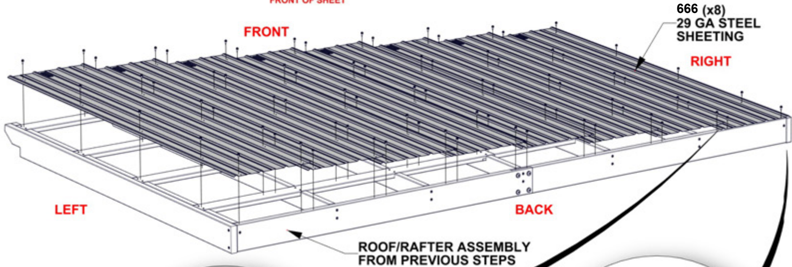
117 (x80) SCREW - 3/4"
