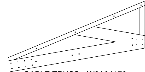
GT1 GABLE TRUSS - W2A04176 (x2) 1 3/8"x34"x64 9/16" (36x854x1640)
