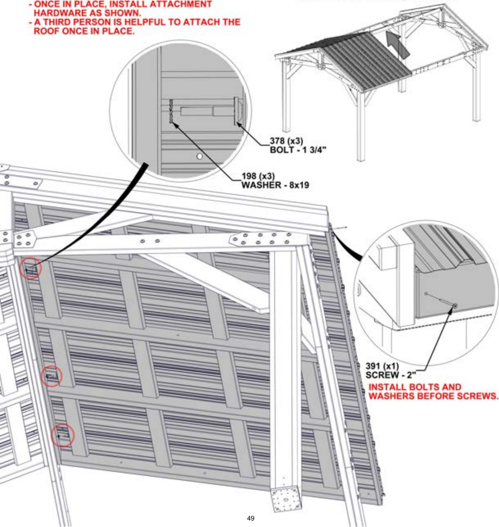
INSTALL ROOF PANEL B, SECTION 1
