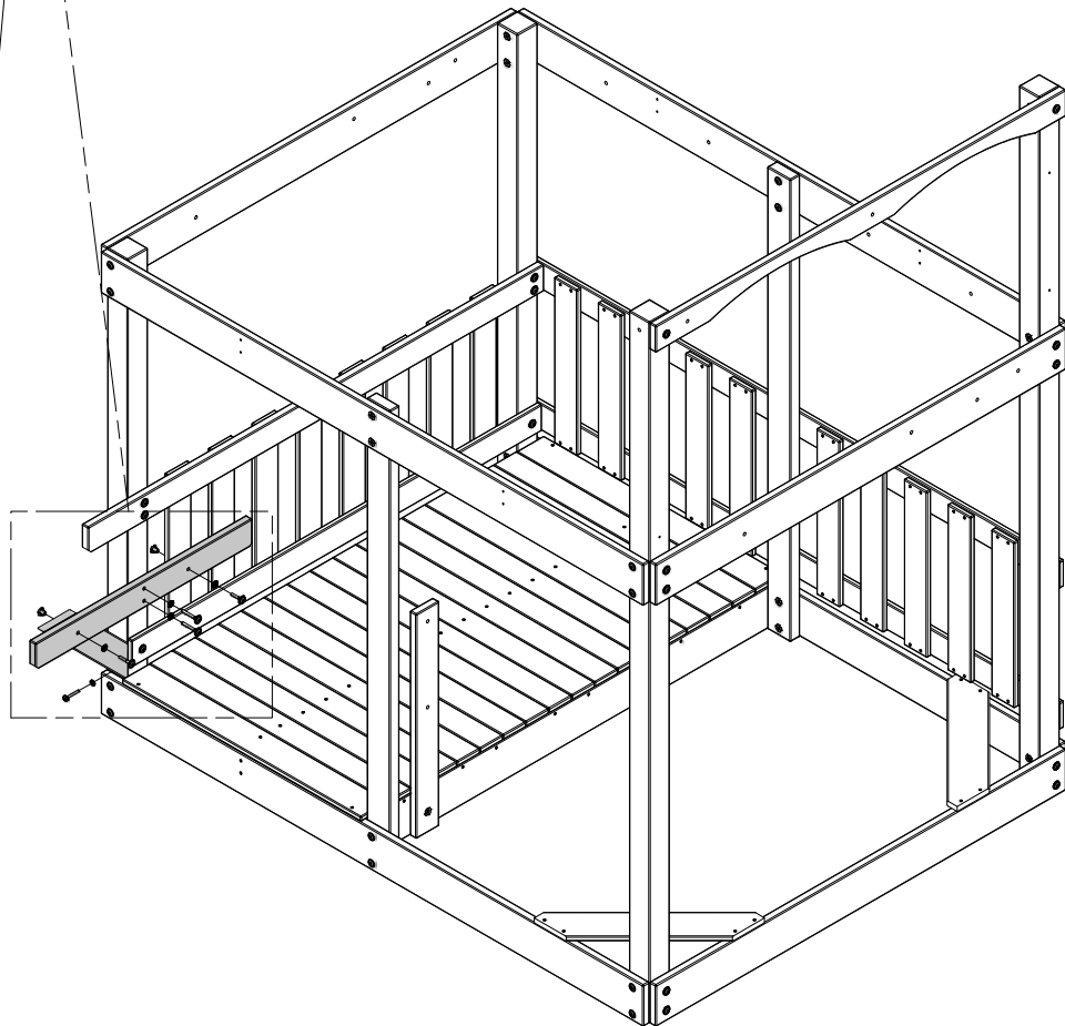
LAG SCREW - 2 1/2"
