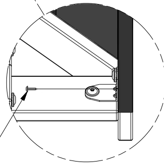
128 (x10) SCREW - 5/8
