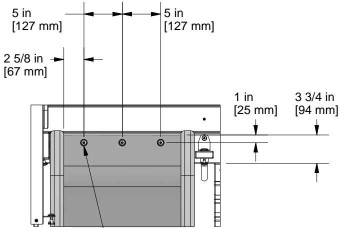
SLIDE ASSEMBLY
