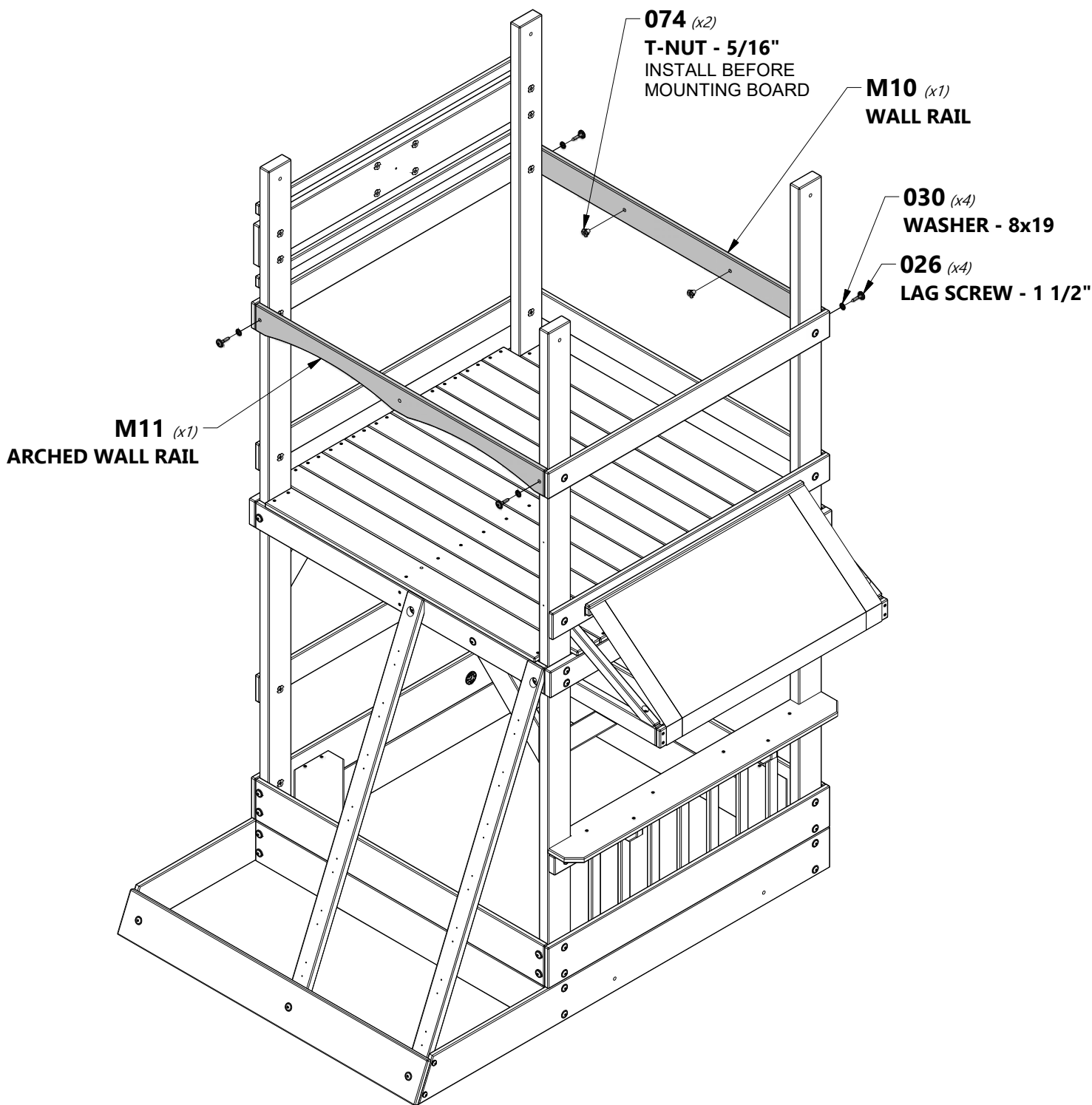
H100074 | T-NUT (2) 5/16"
