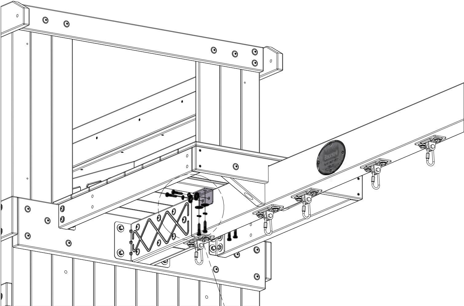
A4M00855 (x2) L BRACKET 51x32x82x3.175
