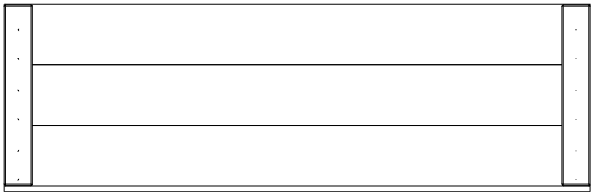
RP2 ROOF PANEL - W2A03794 (x1) 1 5/8"x15 5/8"x59 3/8" (42x396x1241)
