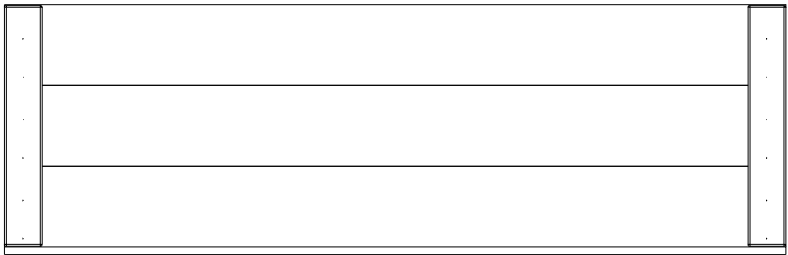
RP2 ROOF PANEL - W2A03794 (x2) 1 5/8"x15 5/8"x59 3/8" (42x396x1241)
