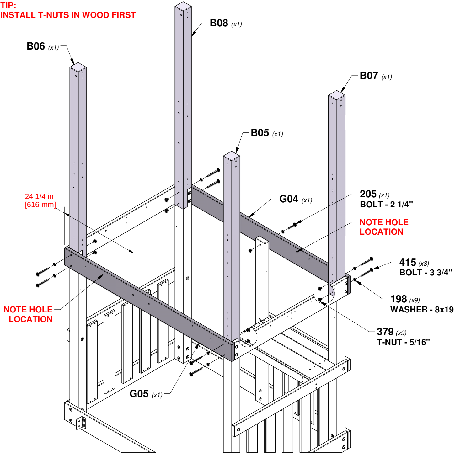
G05 FLOOR RAIL - W4L18951 (x1) 1"x5 1/4"x59" (24x134x1498)
