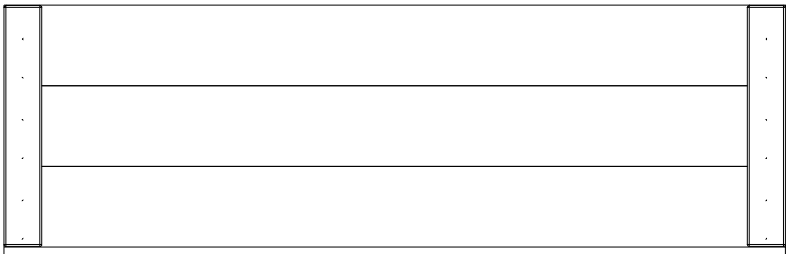
RP2 ROOF PANEL - W2A03794 (x3) 1 5/8"x15 5/8"x59 3/8" (42x396x1241)
