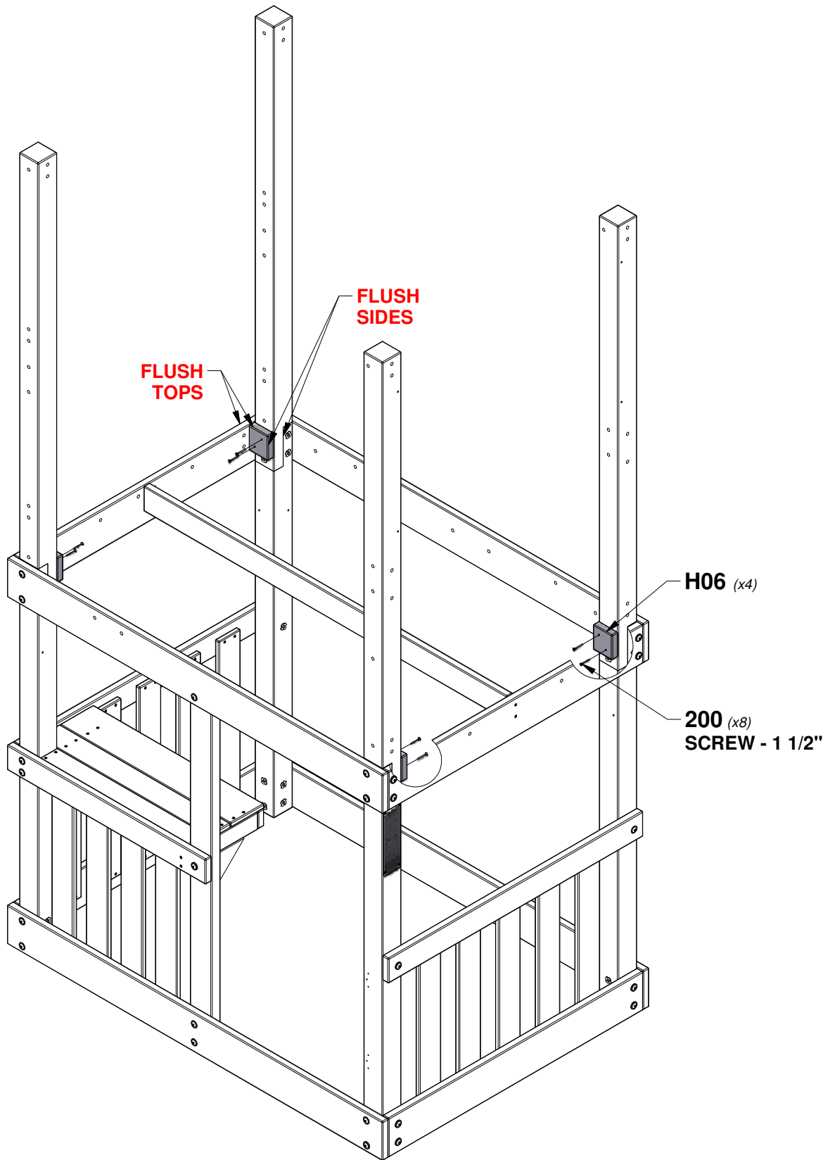
H06 FLOOR BLOCK - W4L18955 (x4) 1"x3"x3 3/8" (24x76x86)
