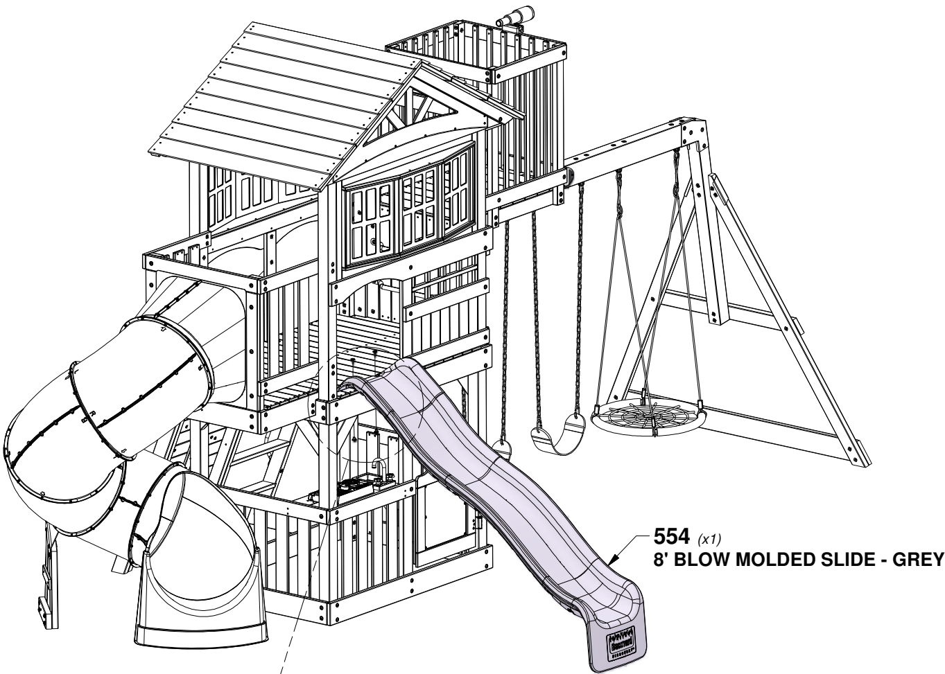
A6P00554 (x1) 8' BLOW MOLDED SLIDE - GREY
