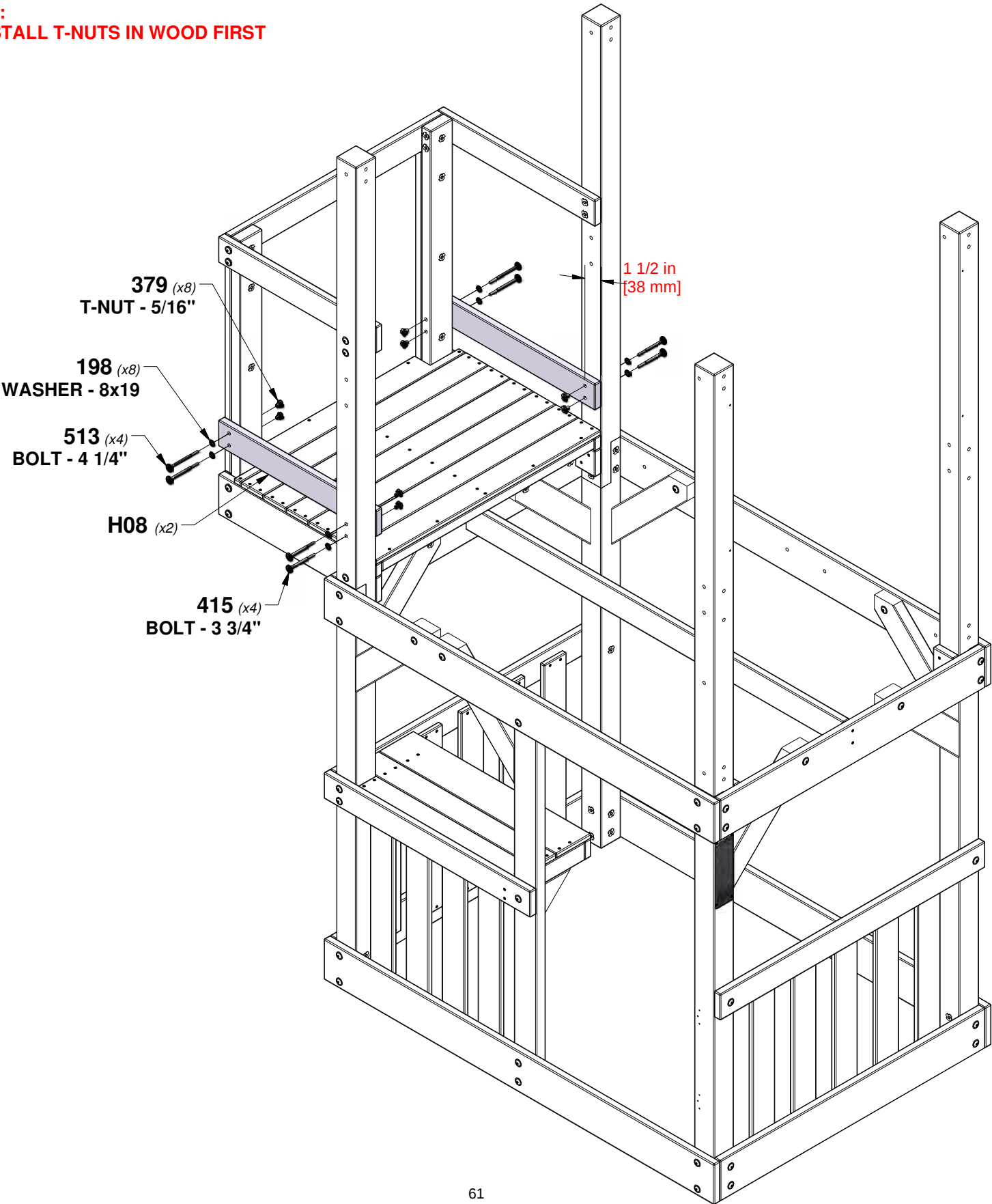
H08 WALL RAIL - W4L18964 (x2) 1"x3 3/8"x23 7/8" (24x86x605)
