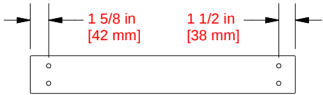
H08 WALL RAIL - W4L18964 (x2) 1"x3 3/8"x23 7/8" (24x86x605)
