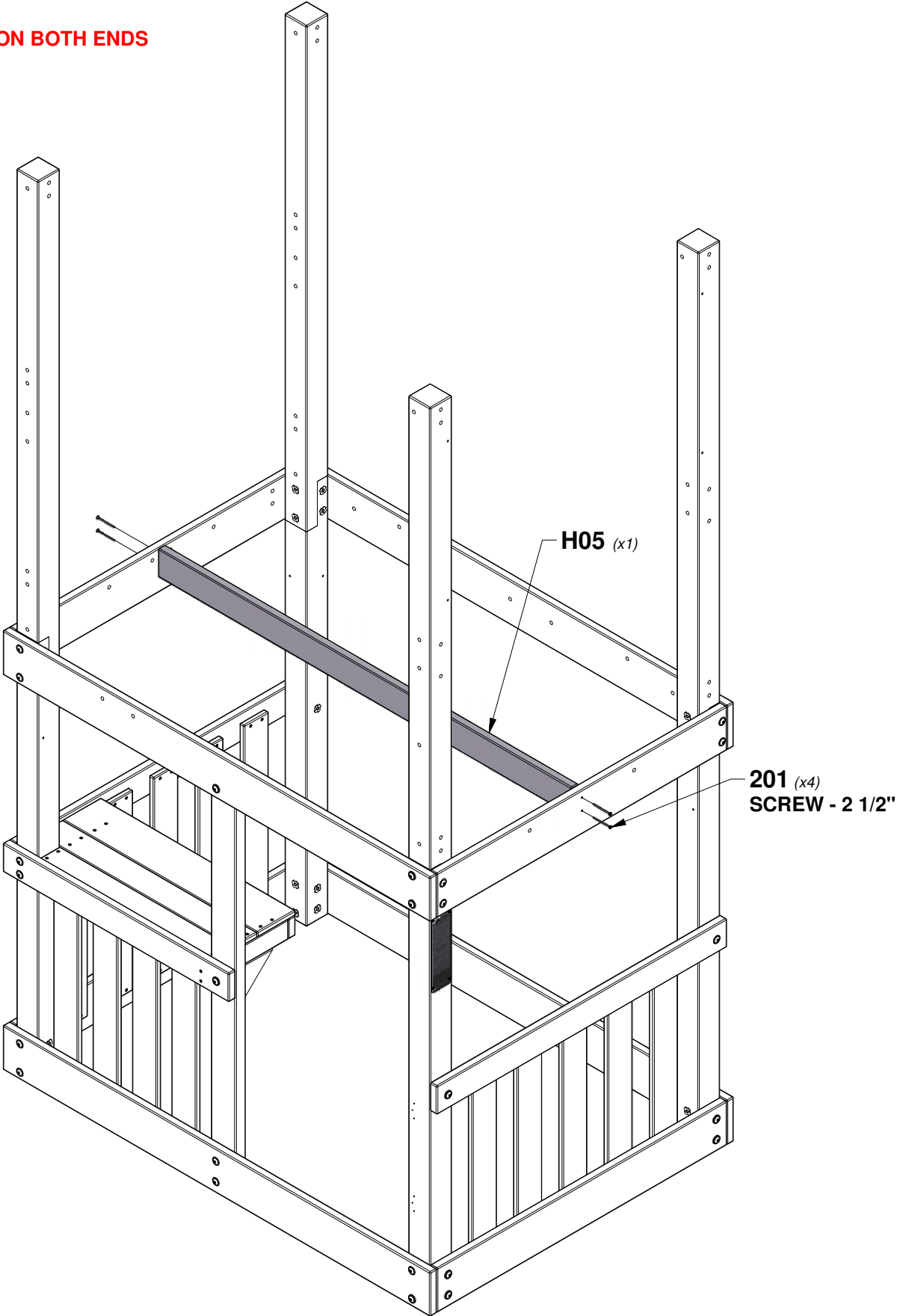
H05 FLOOR JOIST - W4L18954 (x1) 1"x3 3/8"x57 1/8" (24x86x1450)
