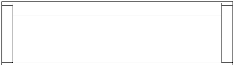
RP1 PEAK ROOF PANEL - W2A03795 (x2) 1 5/8"x13 3/8"x48 7/8" (42x341x1241)
