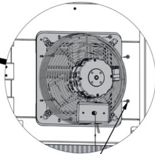
1203 (x8) SCREW - 1 1/4"
