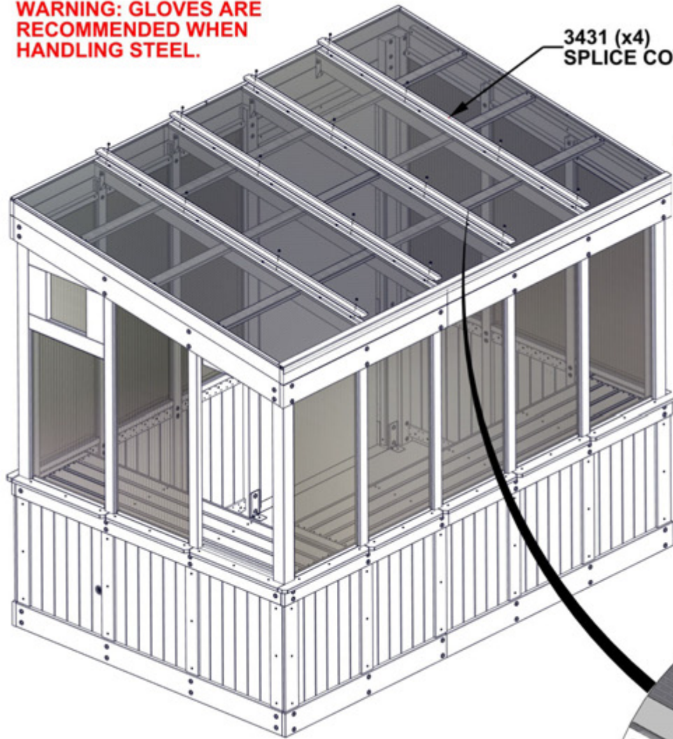
POLY SHEET SPLICE
