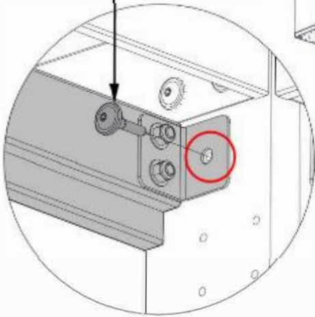
471 (x4) LAG SCREW - 1 1/2"
