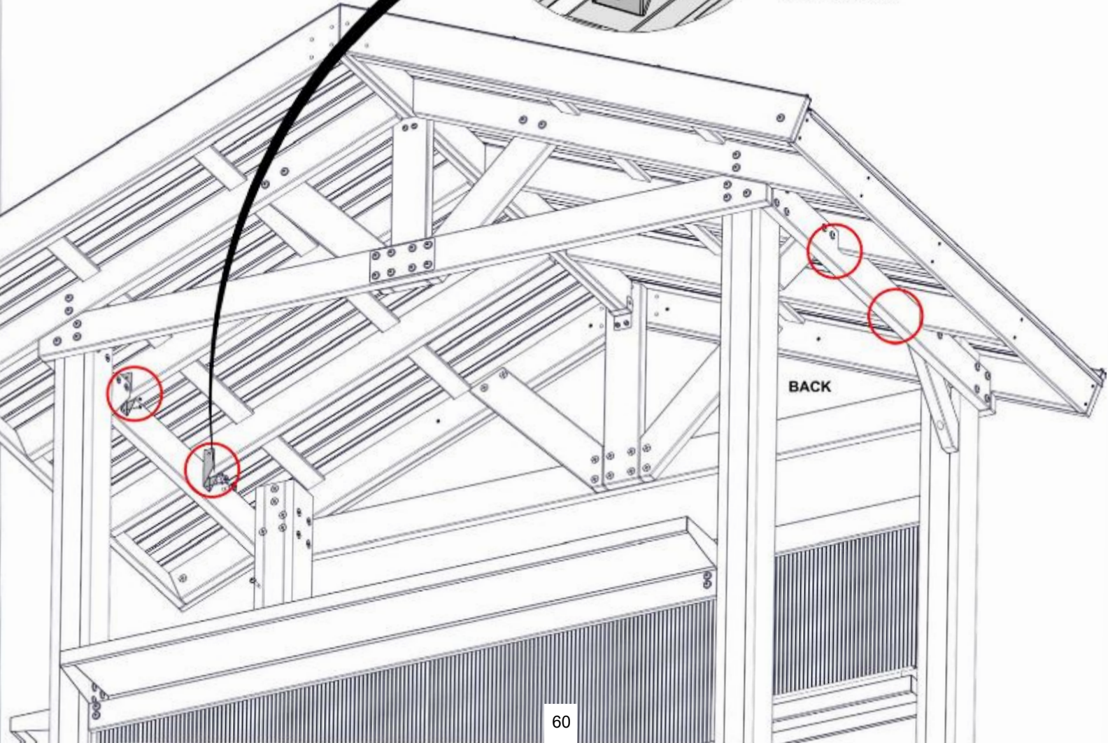
1228 (x4) RAFTER CLIP
