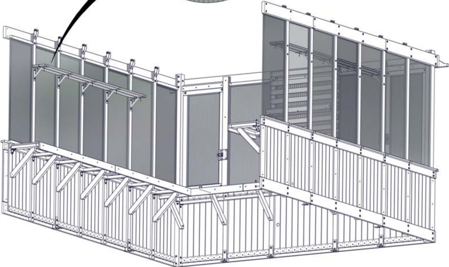
FRONT WALL OF GREENHOUSE NOT SHOWN FOR DETAIL.
