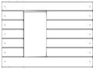
WP07 WALL PANEL - W2A04382 (x2) 1 1/16"x22 1/8"x31 9/16" (27x563x802)
