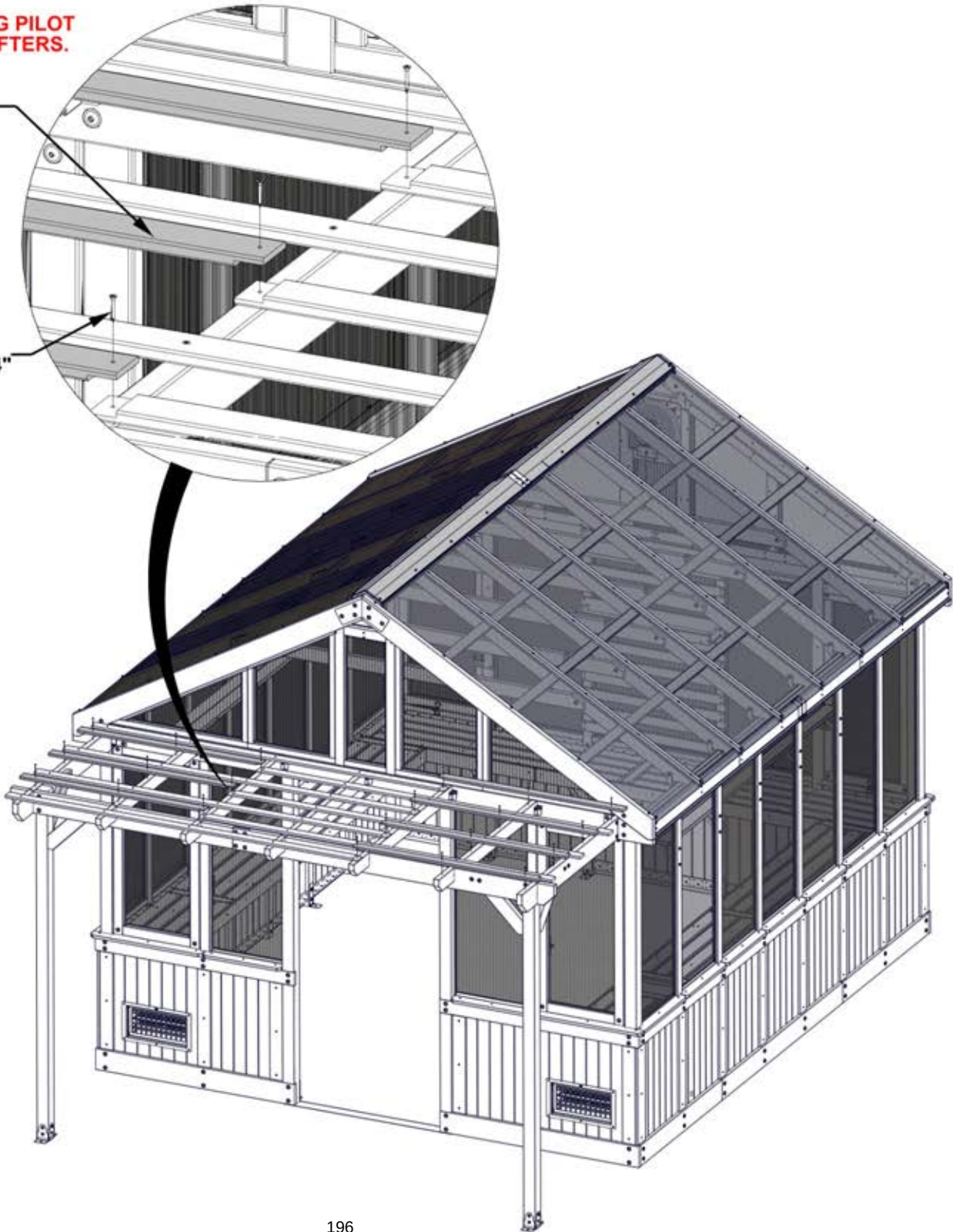
N11 (x7) PERGOLA PURLIN
