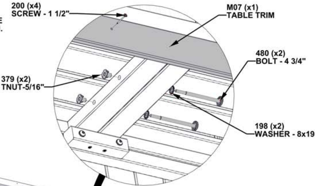
M07 TABLE TRIM - W4L20323 (x1) 5/8"x3 3/8"x44 1/2" (16x86x1131)
