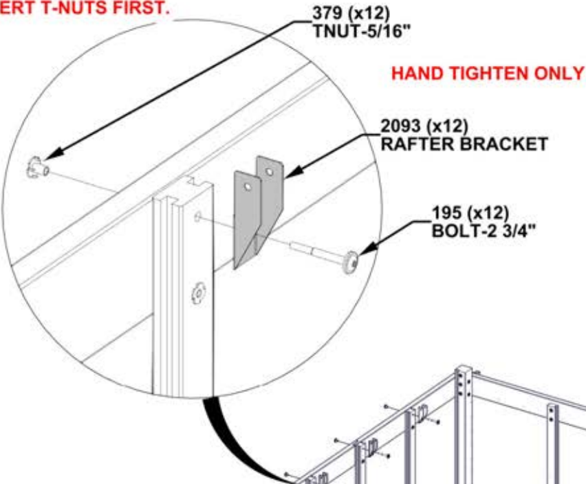
A4M02093 RAFTER BRACKET (x12)
