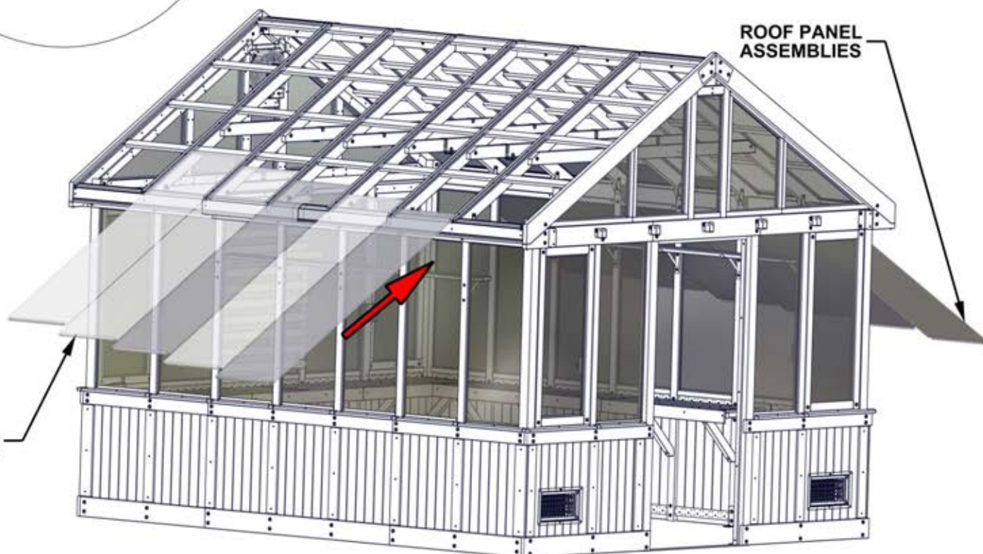
ROOF PANEL ASSEMBLIES
