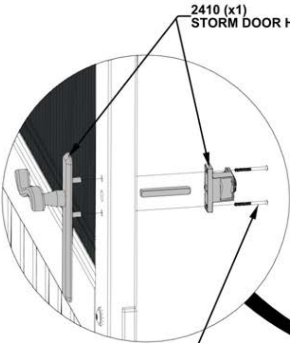
1259 (x2) SCREW - 1 3/4"
