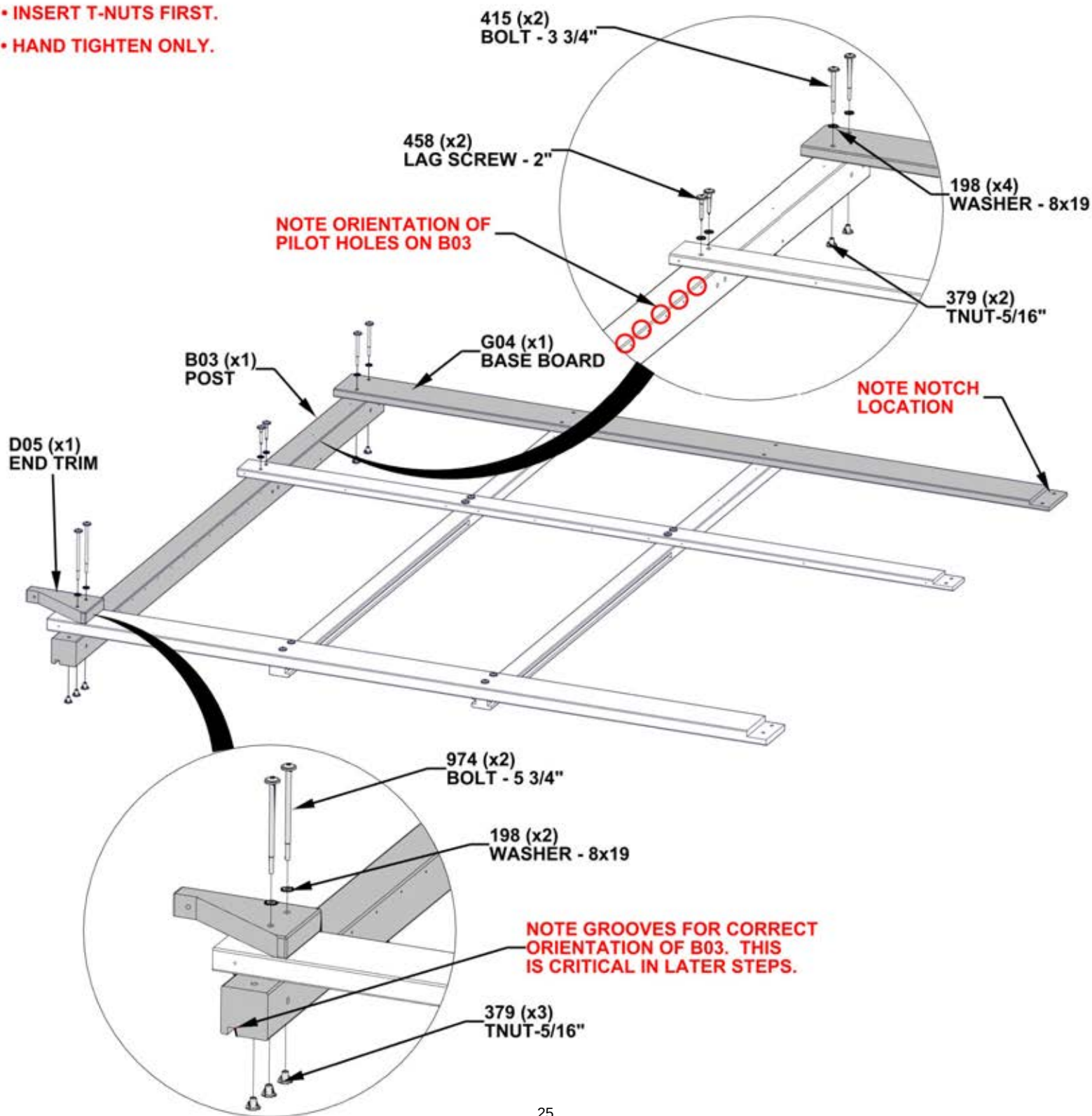
B03 POST - W4L20330 (x1) 3"x3"x88 3/4" (76x76x2254)
