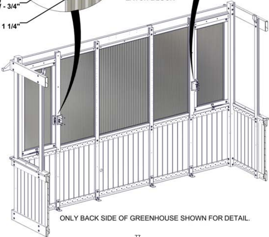
K04 (x2) LATCH BLOCK
