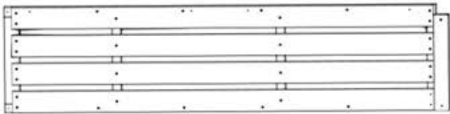
TB05 TABLE ASSEMBLY - W2A04380 (x1) 2 1/16"x16 1/16"x66 13/16" (52x408x1697)
