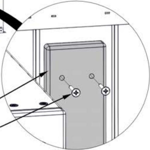
380 (x4) SCREW - 1 1/8"
