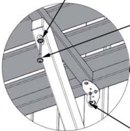
405 (x2) WASHER - 6x15
