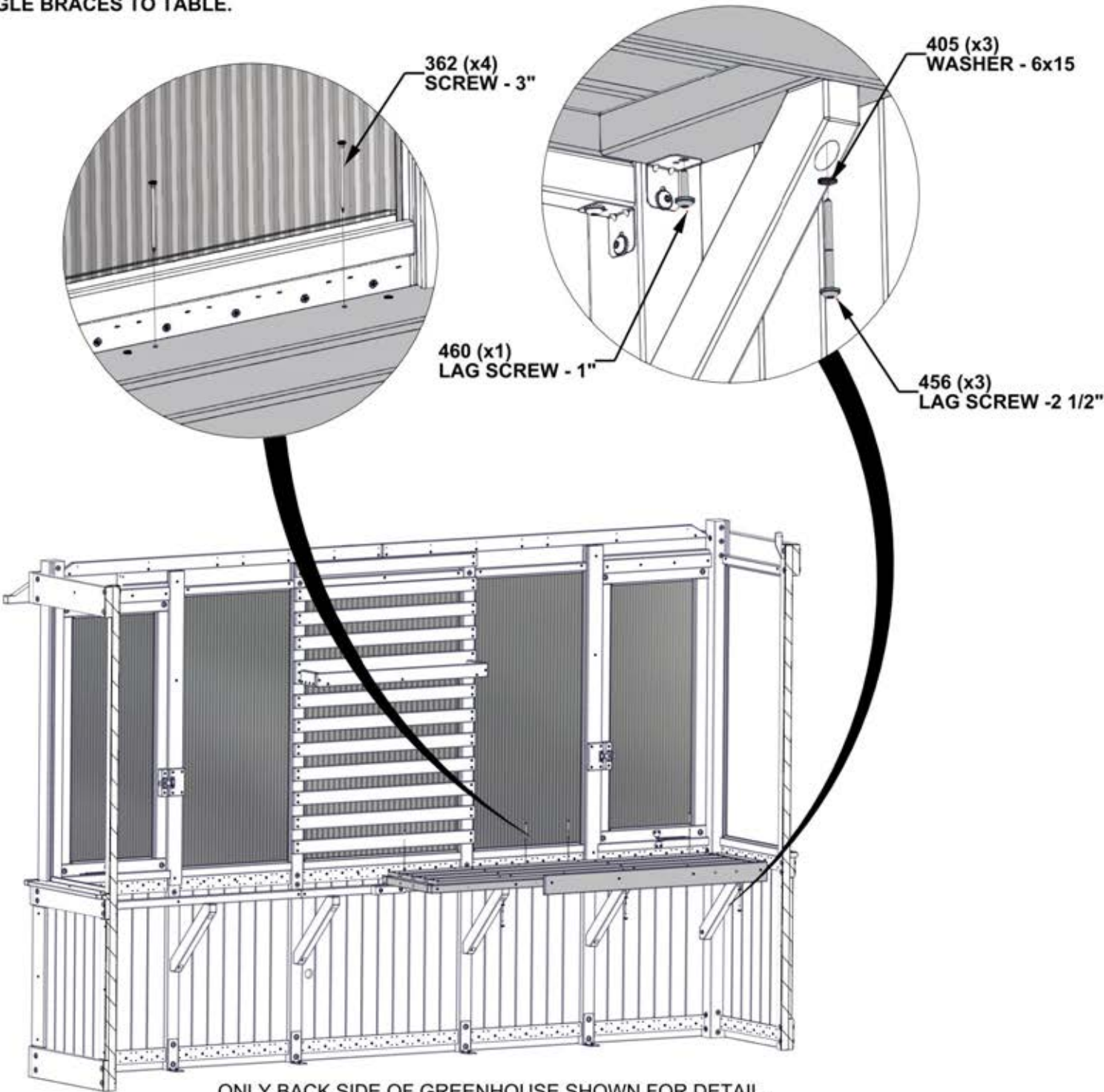
ONLY BACK SIDE OF GREENHOUSE SHOWN FOR DETAIL.
