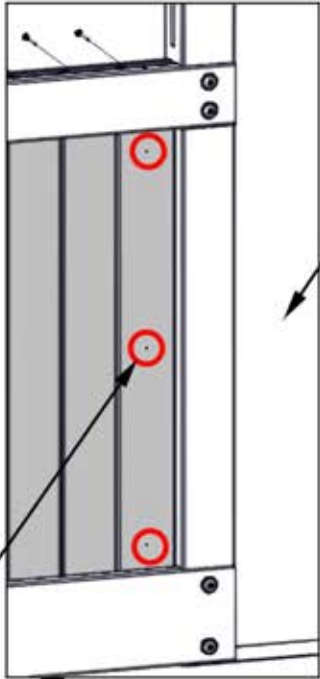
WP07 WALL PANEL - W2A04382 (x2) 1 1/16"x22 1/8"x31 9/16" (27x563x802)
