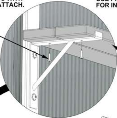
392 (x20) SCREW - 3/4"
