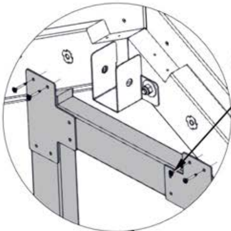
385 (x12) SCREW - 1"
