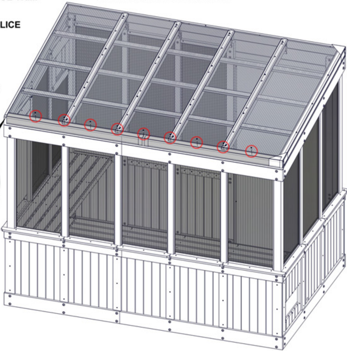
2969 (x2) EDGE TRIM EDGE TRIM PIECES SLIDE INTO SPLICE AND CORNER SPLICE.
