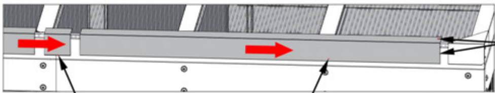
2969 (x2) EDGE TRIM EDGE TRIM PIECES SLIDE INTO SPLICE AND CORNER SPLICE.
