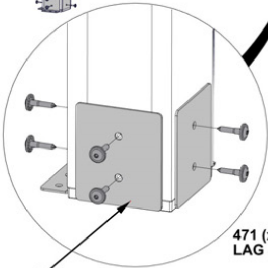
978 (x8) POST PLATE
