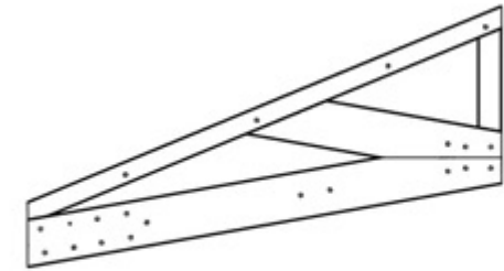
GT1 GABLE TRUSS - W2A03514 (x2) 1 7/16"x29 1/16"x52 9/16" (36x738x1335)
