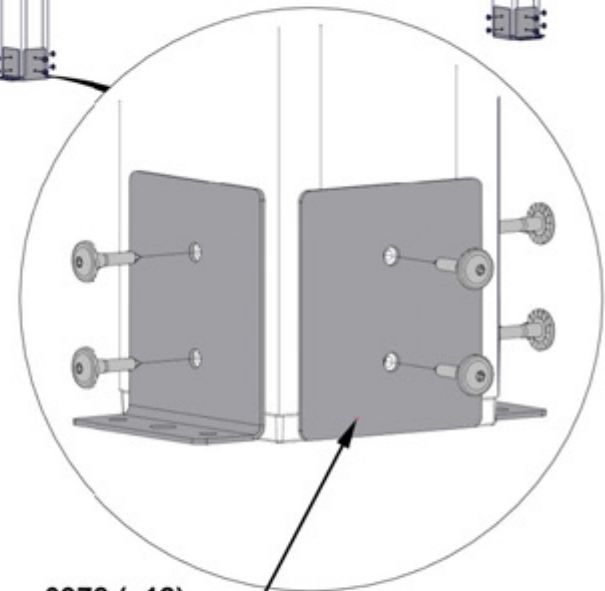
0978 (x12) POST PLATE
