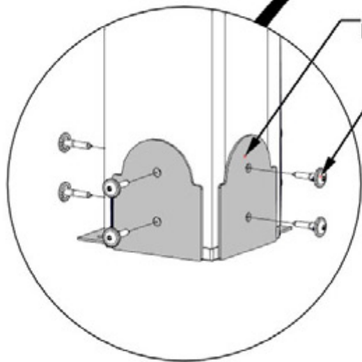
1794(x8) POST PLATE 471 (x32) LAG SCREW - 1 1/2"
