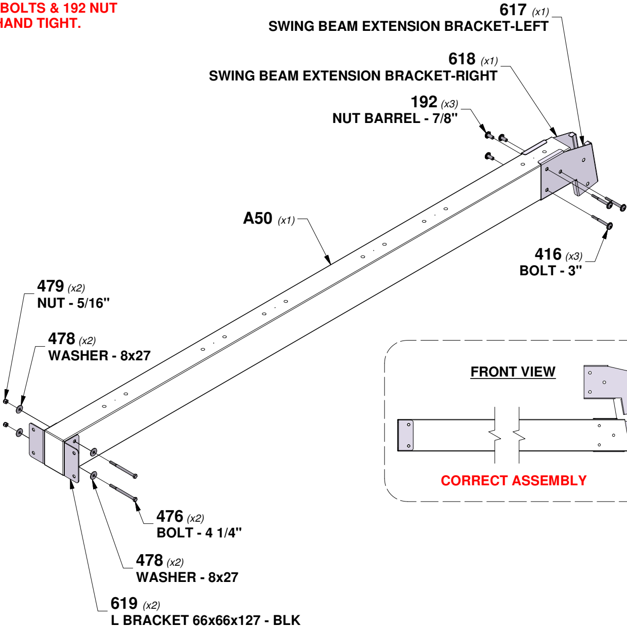
A4M00617 SWING BEAM EXTENSION BRACKET-LEFT (x1)
