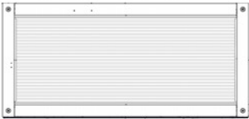
WA07 WINDOW ASSEMBLY - W2A04206 (x1) 1 7/8"x21 13/16"x47 3/16" (48x554x1094)
