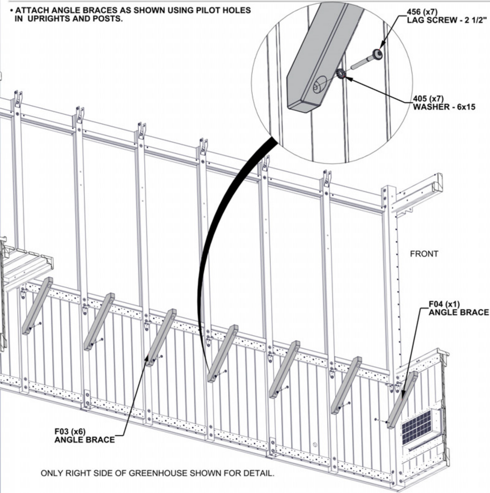
F04 ANGLE BRACE - W4L19488 (x1) 1 7/16"x2 3/8"x18 1/16" (36x60x458)
