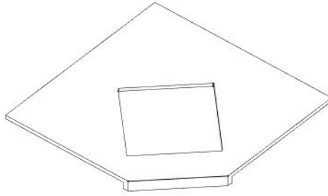
M14 CABINET MARBLE - A4M04712 (x1) 36"x36"x1 15/16" (50x914x914)
