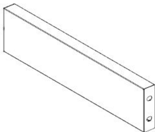
H4 CABINET HORIZONTAL BEAM ASSEMBLY - A4M04719 (x1) 14 5/8"x3 3/8"x1" (25x85x372)
