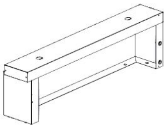
T5 CABINET MARBLE PANEL ASSEMBLY L - A4M04537 (x1) 24 1/8"x4 5/16"x6 3/4" (109x172.2x612)
