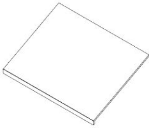
M13 CABINET MARBLE - A4M04711 (x1) 28 1/8"x24 15/16"x1 15/16" (50x634x715)
