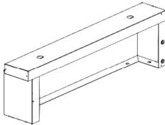
T5 CABINET MARBLE PANEL ASSEMBLY L - A4M04537 (x1) 24 1/8"x4 5/16"x6 3/4" (109x172.2x612)
