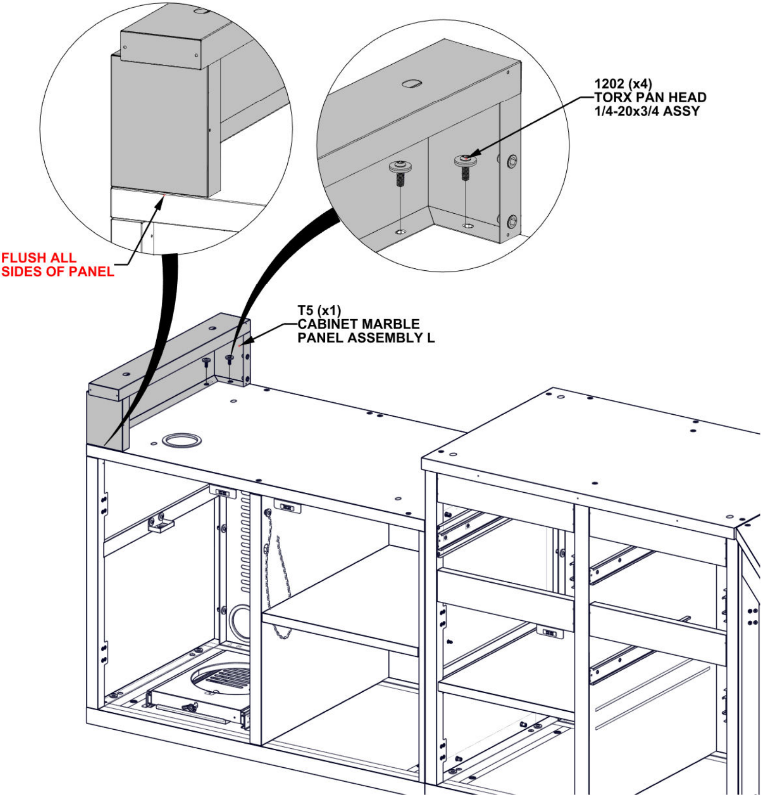
T5 CABINET MARBLE PANEL ASSEMBLY L - A4M04537 (x1) 24 1/8"x4 5/16"x6 3/4" (109x172.2x612)
