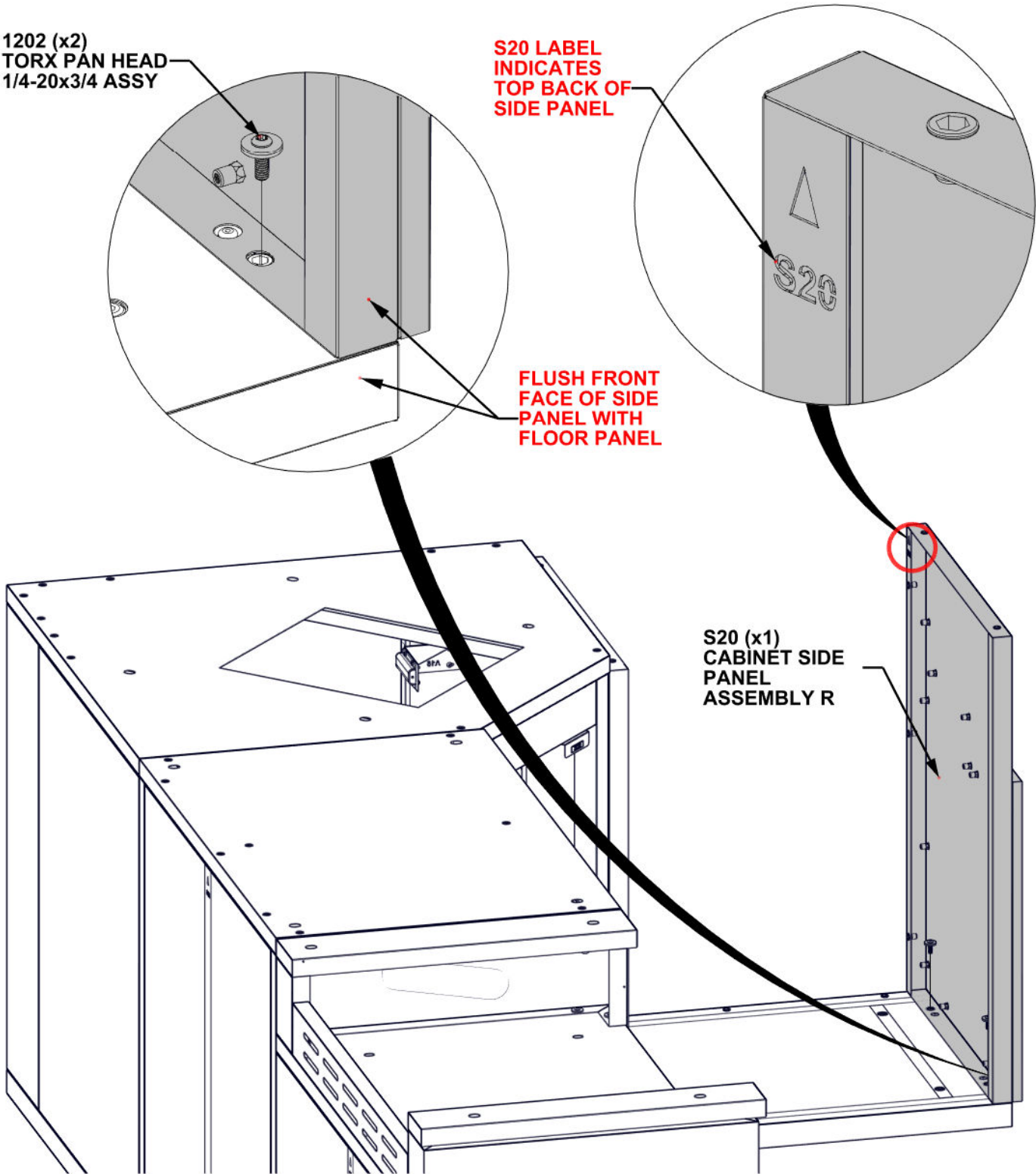
S20 CABINET SIDE PANEL ASSEMBLY R - A4M04669 (x1) 33 3/8"x23 3/8"x2 1/16" (53.00x594x848.20)
