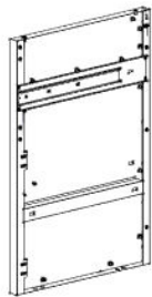
S36 CABINET SIDE PANEL ASSEMBLY L - A4M04852 (x1) 33 3/8"x23 3/8"x1 3/8" (35.00x594.00x848.20)
