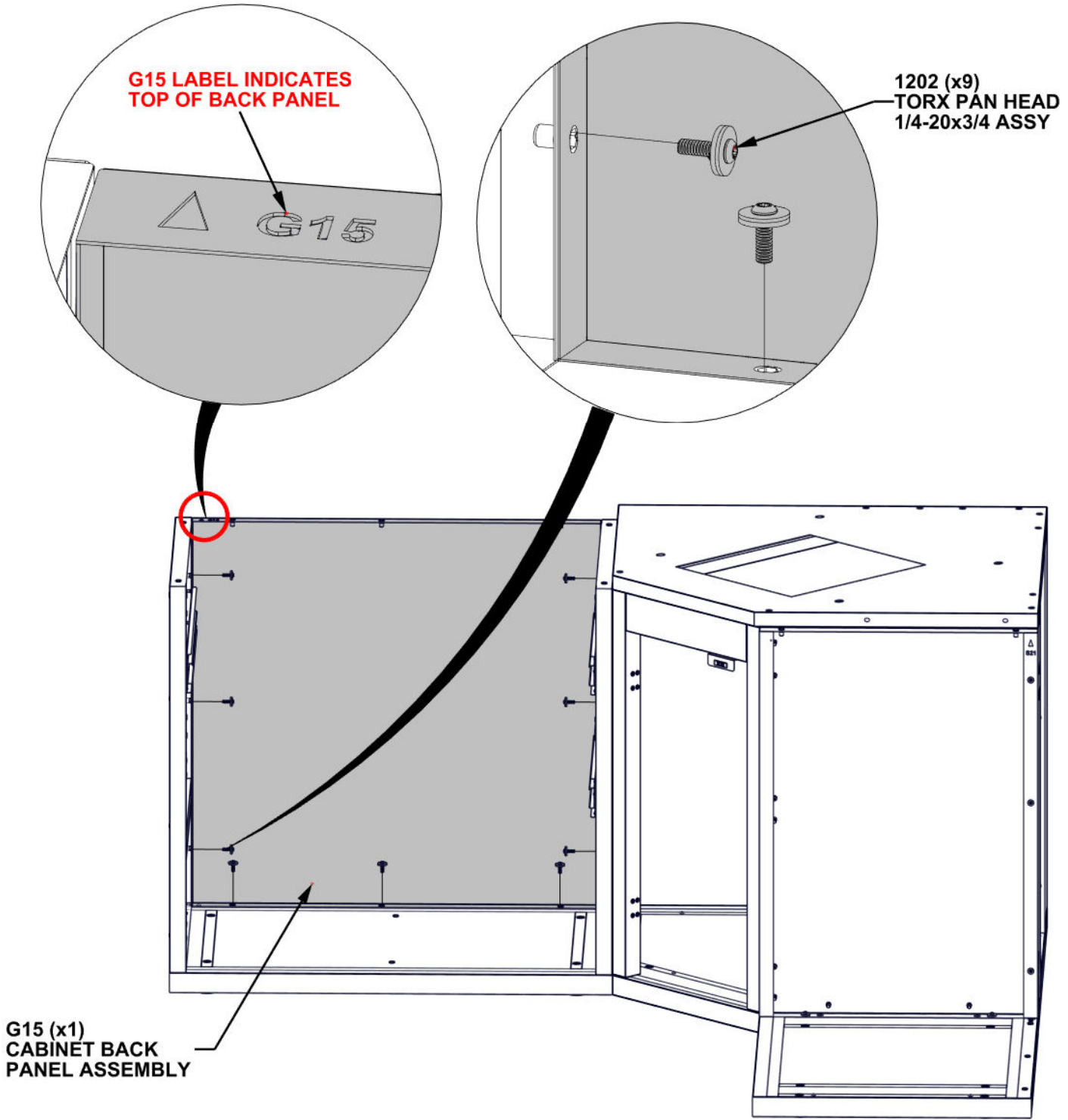
G15 CABINET BACK PANEL ASSEMBLY - A4M04707 (x1) 34 5/16"x33 3/8"x1 3/16" (30x847.2x1049)
