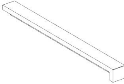
M11 CABINET MARBLE - A4M04663 (x1) 24 15/16"x2 1/16"x11/16" (18.00x53.00x634.00)
