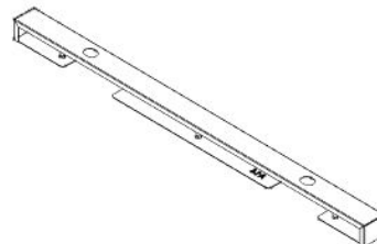
A14 MARBLE BRACKET ASSEMBLY - A4M04846 (x1) 24 3/16"x1 3/8"x1 1/4" (31.00x35.00x614.00)
