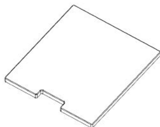
M5 SINK COVER MARBLE - A4M03147 (x1) 11/16"x14 3/4"x16 5/16" (18x375x415)
