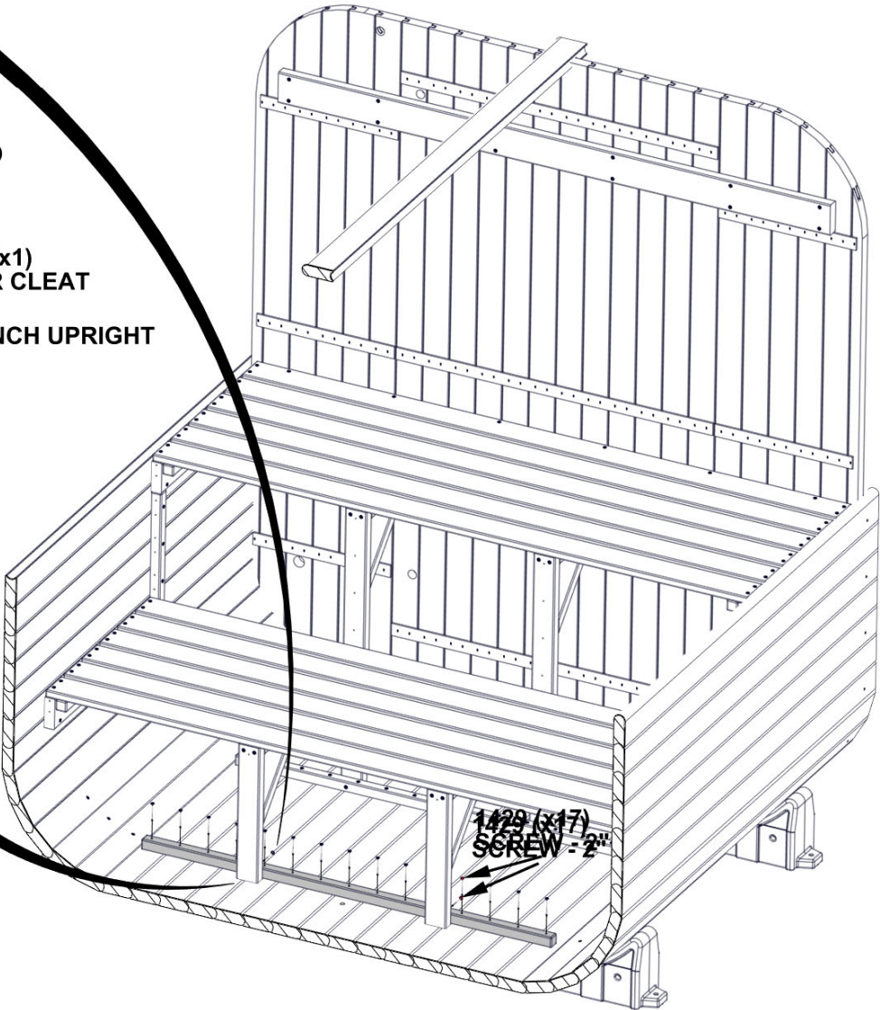
VIEW FROM UNDERNEATH BENCH AND BEHIND BENCH UPRIGHT
