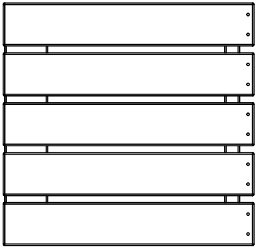
BA03 BENCH ASSEMBLY-W2A04824 (x1) 1 15/16"x19 1/8"x19 3/4" (50x486x502)
