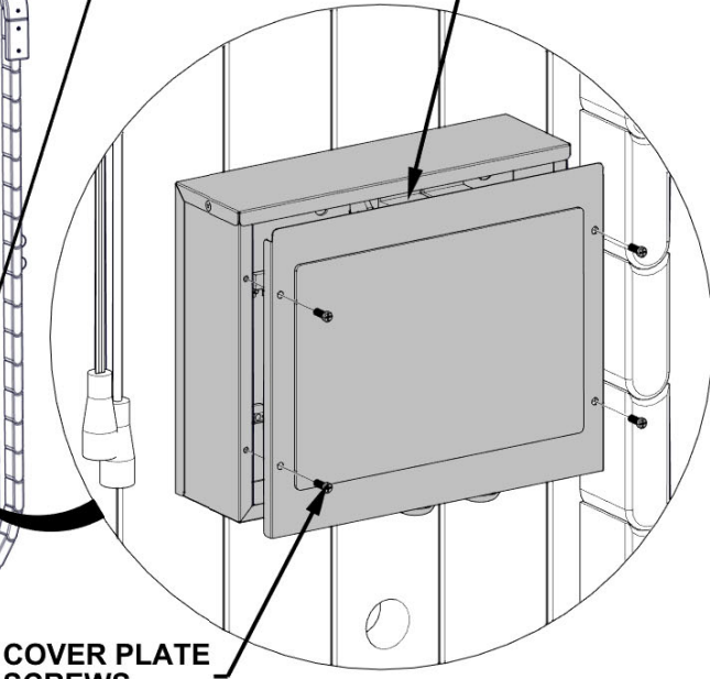
COVER PLATE
