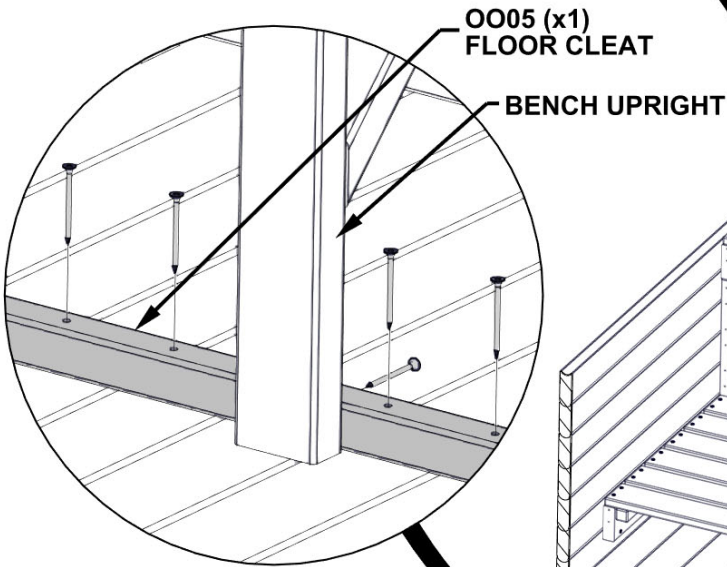
VIEW FROM UNDERNEATH BENCH AND BEHIND BENCH UPRIGHT
