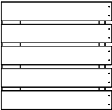
BA04 BENCH ASSEMBLY-W2A04825 (x1) 1 15/16"x17 15/16"x19 3/4" (50x456x502)
