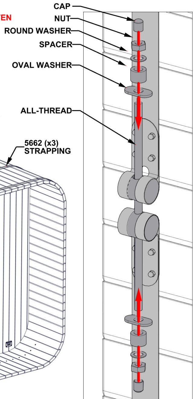
4TH STRAP
