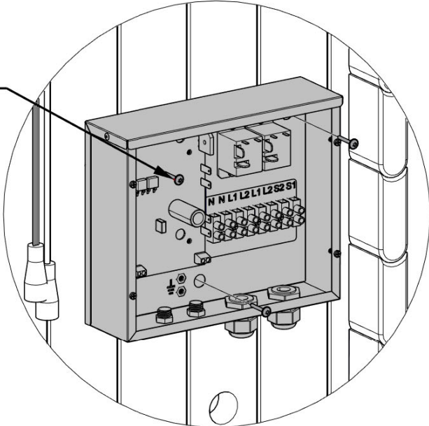
1440 (x3) SCREW - 1"
