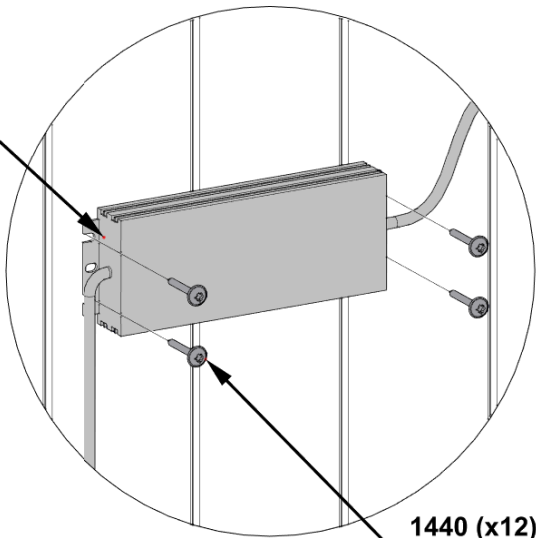
1440 (x12) SCREW - 1"
