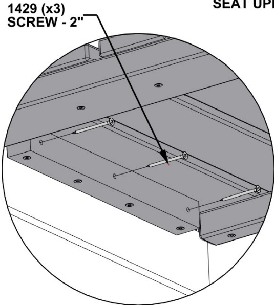
DETAIL 'C'
