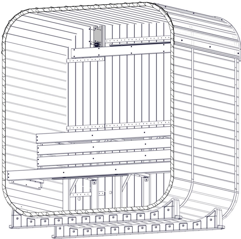
FRONT OF SAUNA HIDDEN FOR DETAIL
