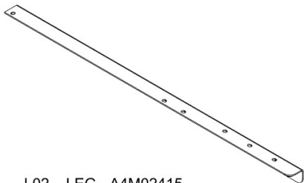
L02 LEG - A4M02415 (x1) 1 1/2"x1 1/2"x31 13/16" (38x38x808)
