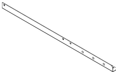
L03 LEG - A4M02416 (x1) 1 1/2"x1 1/2"x31 13/16" (38x38x808)
