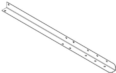
L04 LEG - A4M02417 (x1) 3 3/4"x4 3/4"x31 15/16" (95x120x811)
