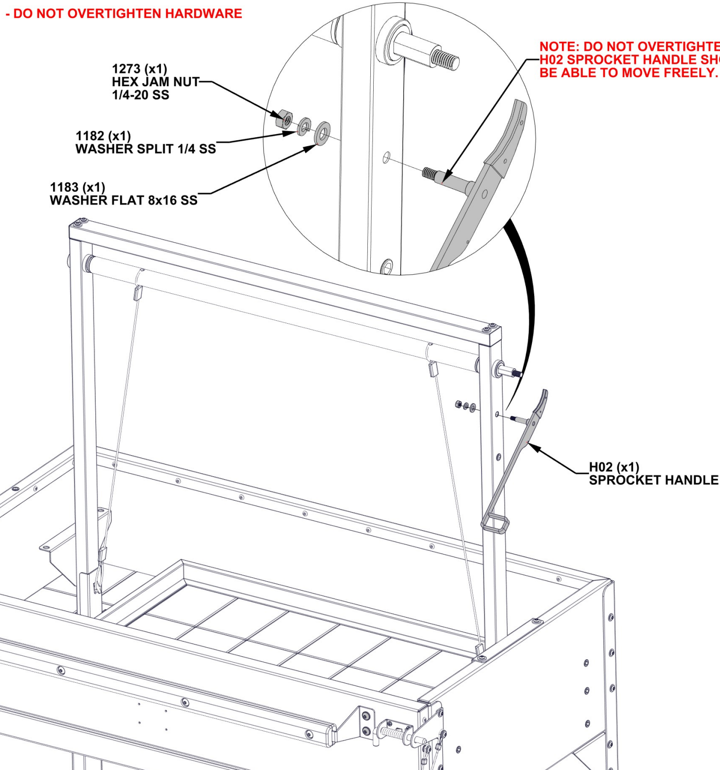
H02 SPROCKET HANDLE - A4M02497 (x1) 7/8"x3 5/8"x11 1/4" (22x92x285)
