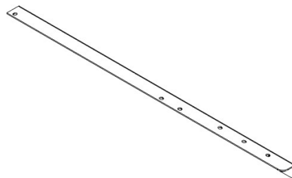
L02 LEG - A4M02415 (x1) 1 1/2"x1 1/2"x31 13/16" (38x38x808)
