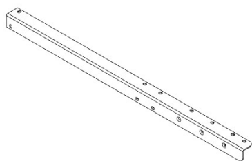
L01 LEG - A4M02414 (x1) 1 1/2"x1 1/2"x31 13/16" (38x38x808)
