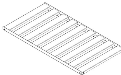
B02 BOTTOM RACK ASSEMBLY - A4M02142 (x1) 1 5/8"x24 1/16"x 45 1/16" (40.5x611.5x1144.5)
