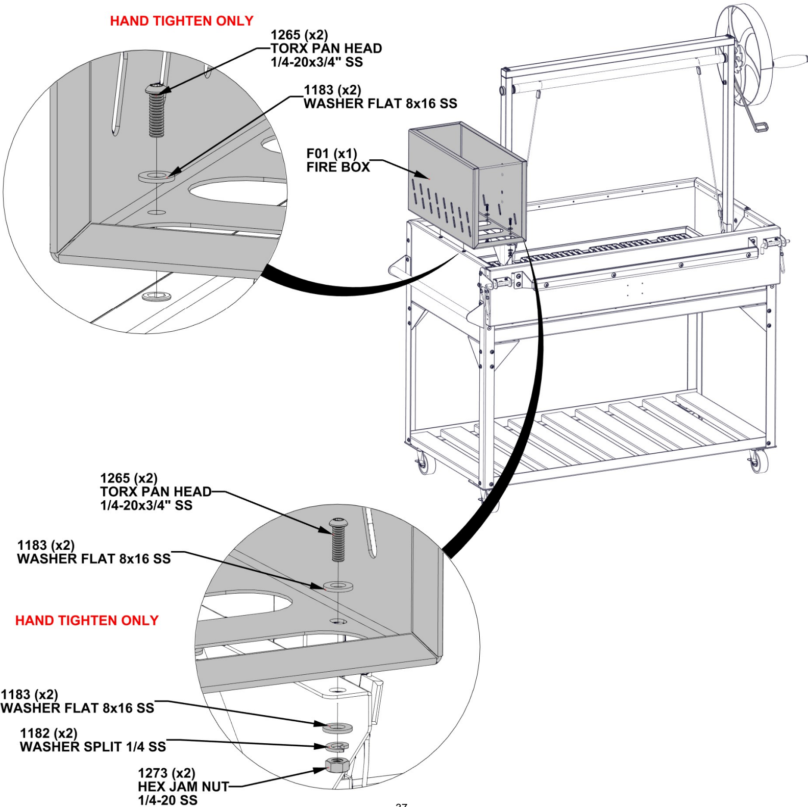
F01 FIRE BOX - A4M02151 (x1) 8 1/4"x11 11/16"x20 1/16" (210x298x510)
