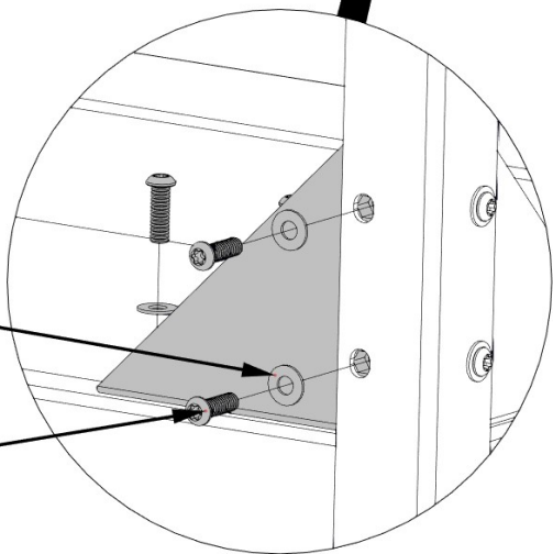
B04 (x4) LEG BRACE
