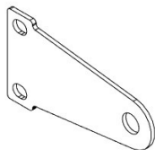
B03 LATCH BRACKET - A4M02413 (x2) 1/8"x2 3/16"x4 1/8" (2.5x56x104)
