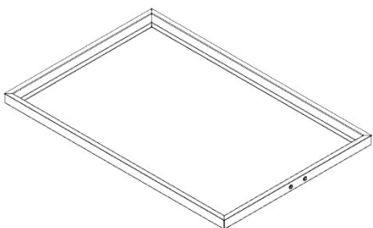
G01 GRATE TRAY ASSEMBLY - A4M02144 (x1) 1 1/4"x 21 13/16"x33 1/16" (31.8x554x839)
