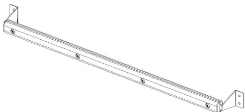
H01 DOOR HANDLE ASSEMBLY - A4M02412 (x1) 2 3/8"x3 3/4"x37 7/16" (60x95x951)
