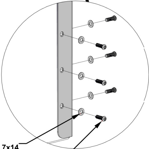
1264 (x6) TORX PAN HEAD 1/4-20x3/4" BLK
