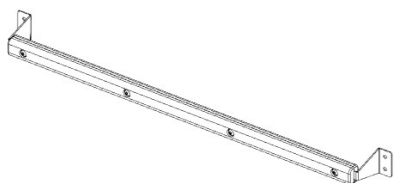
H01 DOOR HANDLE ASSEMBLY - A4M02412 (x1) 2 3/8"x3 3/4"x37 7/16" (60x95x951)
