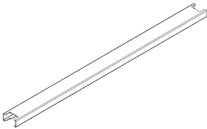
R01 REMOVABLE BOTTOM RAIL - A4M02871 (x1) 1 1/16"x2 3/8"x35" (27.5x60x889)
