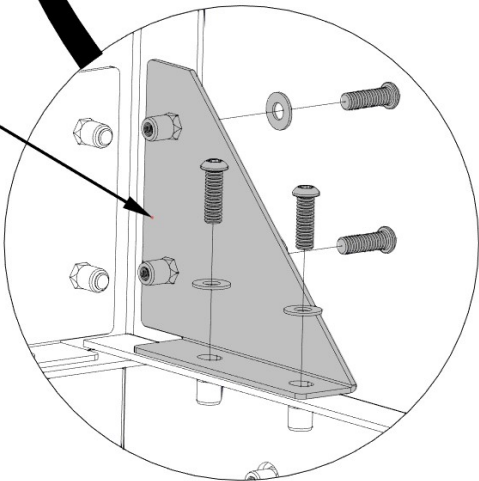
B04 (x4) LEG BRACE
