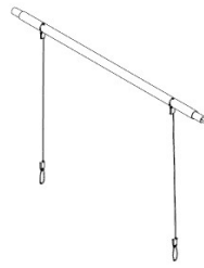
S01 SPINDLE ASSEMBLY - A4M02150 (x1) 1 3/16"x37 1/2" (30x955)
