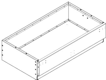
C01 COAL PAN ASSEMBLY - A4M02135 (x1) 2"x25 1/4"x44 13/16" (292x642x1139)
