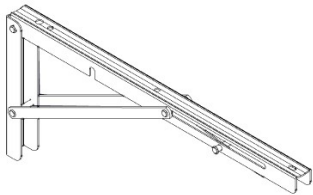
2094 TABLE BRACKET - A4M02094 (x2) 1 3/8"x6 13/16"x15 15/16" (34x173x405)
