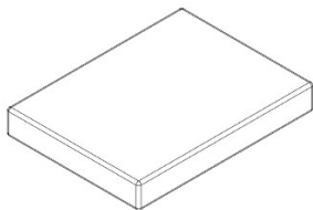
0729 FIRE BRICK - A6P00729 (x40) 13/16"x4 3/16"x5 9/16" (20x107x142)
